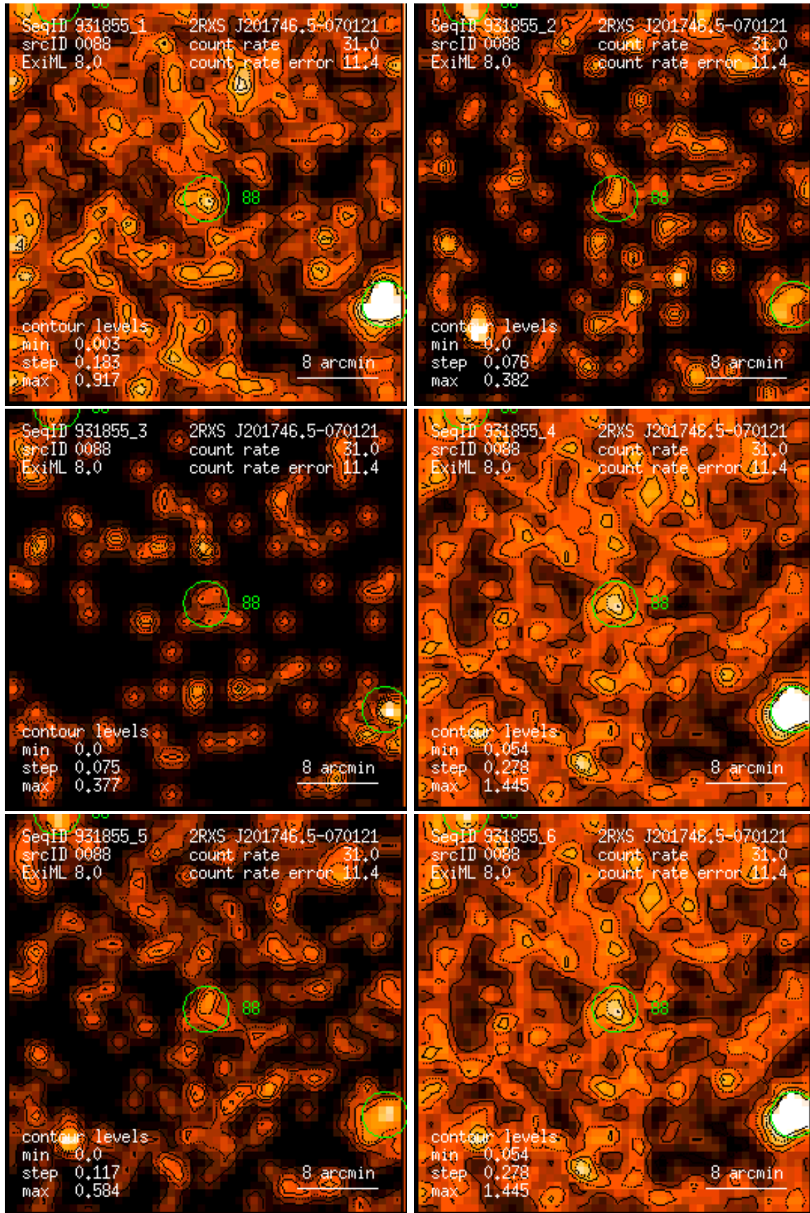
Figure 88: RASS 931855: detection 0088: band rate images, Gaussian filter: (1) PSPC channels 11 – 41, (2) 52 – 90, (3) 91 – 201, (4) 11 – 235, (5) 52 – 201, (6) 11 – 201. Broad band rates in counts/ks. Band rate contour levels in counts/ks/arcmin 2 .
