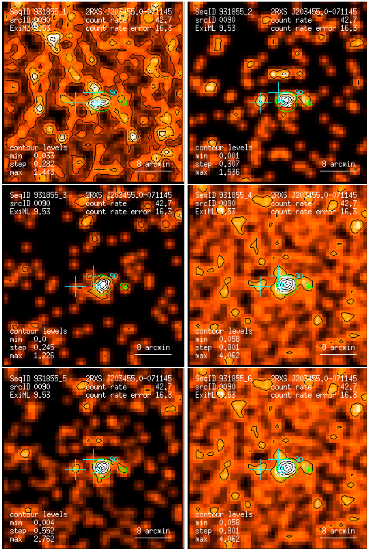
Figure 90: RASS 931855: detection 0090: band rate images, Gaussian filter: (1) PSPC channels 11 – 41, (2) 52 – 90, (3) 91 – 201, (4) 11 – 235, (5) 52 – 201, (6) 11 – 201. Broad band rates in counts/ks. Band rate contour levels in counts/ks/arcmin 2 .
