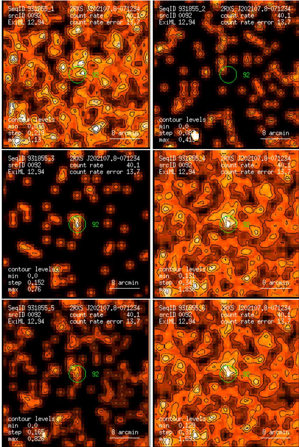
Figure 92: RASS 931855: detection 0092: band rate images, Gaussian filter: (1) PSPC channels 11 – 41, (2) 52 – 90, (3) 91 – 201, (4) 11 – 235, (5) 52 – 201, (6) 11 – 201. Broad band rates in counts/ks. Band rate contour levels in counts/ks/arcmin 2 .
