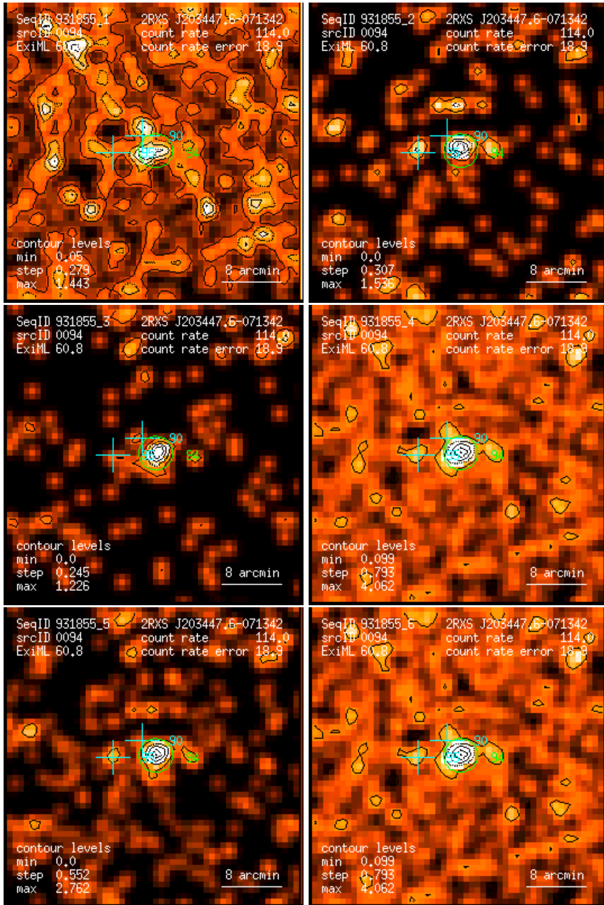
Figure 94: RASS 931855: detection 0094: band rate images, Gaussian filter: (1) PSPC channels 11 – 41, (2) 52 – 90, (3) 91 – 201, (4) 11 – 235, (5) 52 – 201, (6) 11 – 201. Broad band rates in counts/ks. Band rate contour levels in counts/ks/arcmin 2 .
