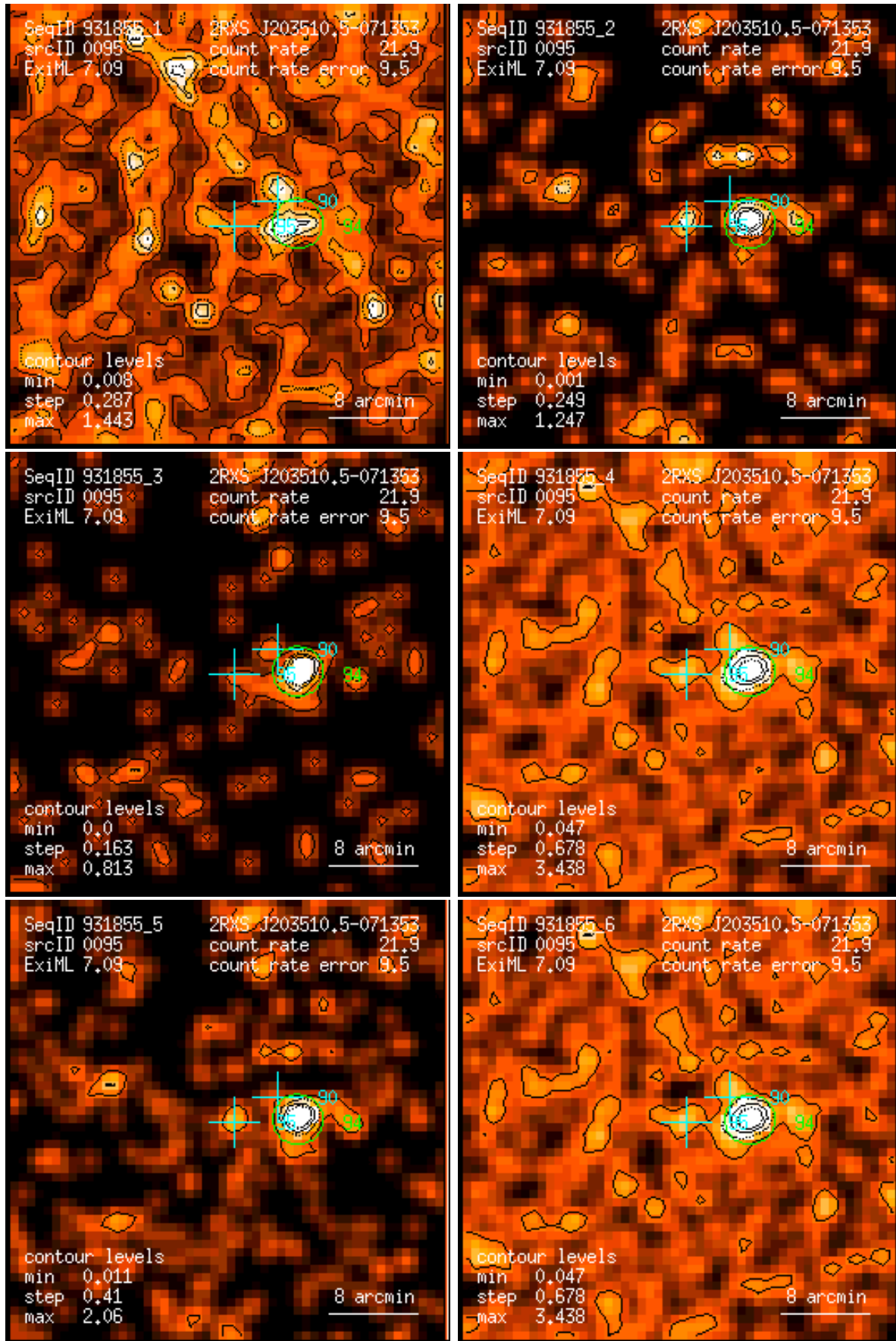
Figure 95: RASS 931855: detection 0095: band rate images, Gaussian filter: (1) PSPC channels 11 – 41, (2) 52 – 90, (3) 91 – 201, (4) 11 – 235, (5) 52 – 201, (6) 11 – 201. Broad band rates in counts/ks. Band rate contour levels in counts/ks/arcmin 2 .
