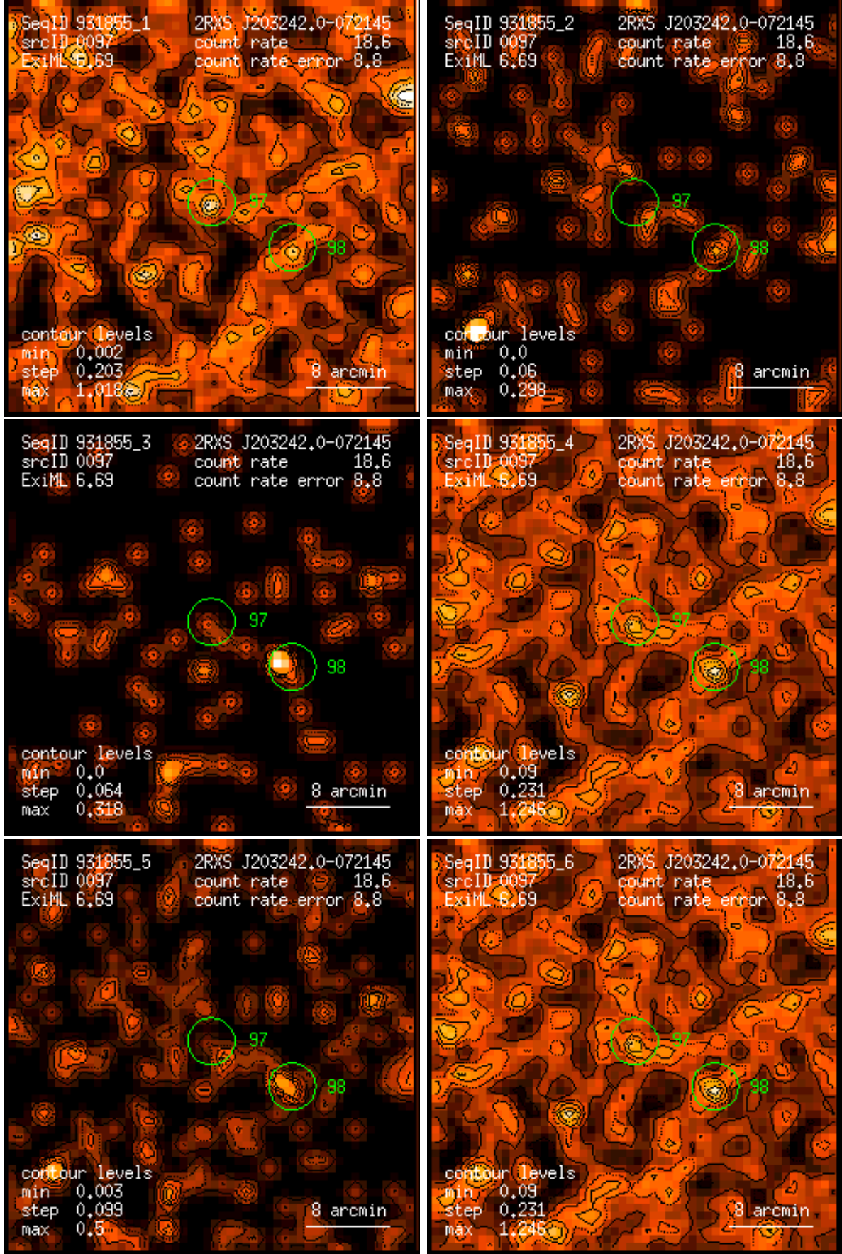
Figure 97: RASS 931855: detection 0097: band rate images, Gaussian filter: (1) PSPC channels 11 – 41, (2) 52 – 90, (3) 91 – 201, (4) 11 – 235, (5) 52 – 201, (6) 11 – 201. Broad band rates in counts/ks. Band rate contour levels in counts/ks/arcmin 2 .
