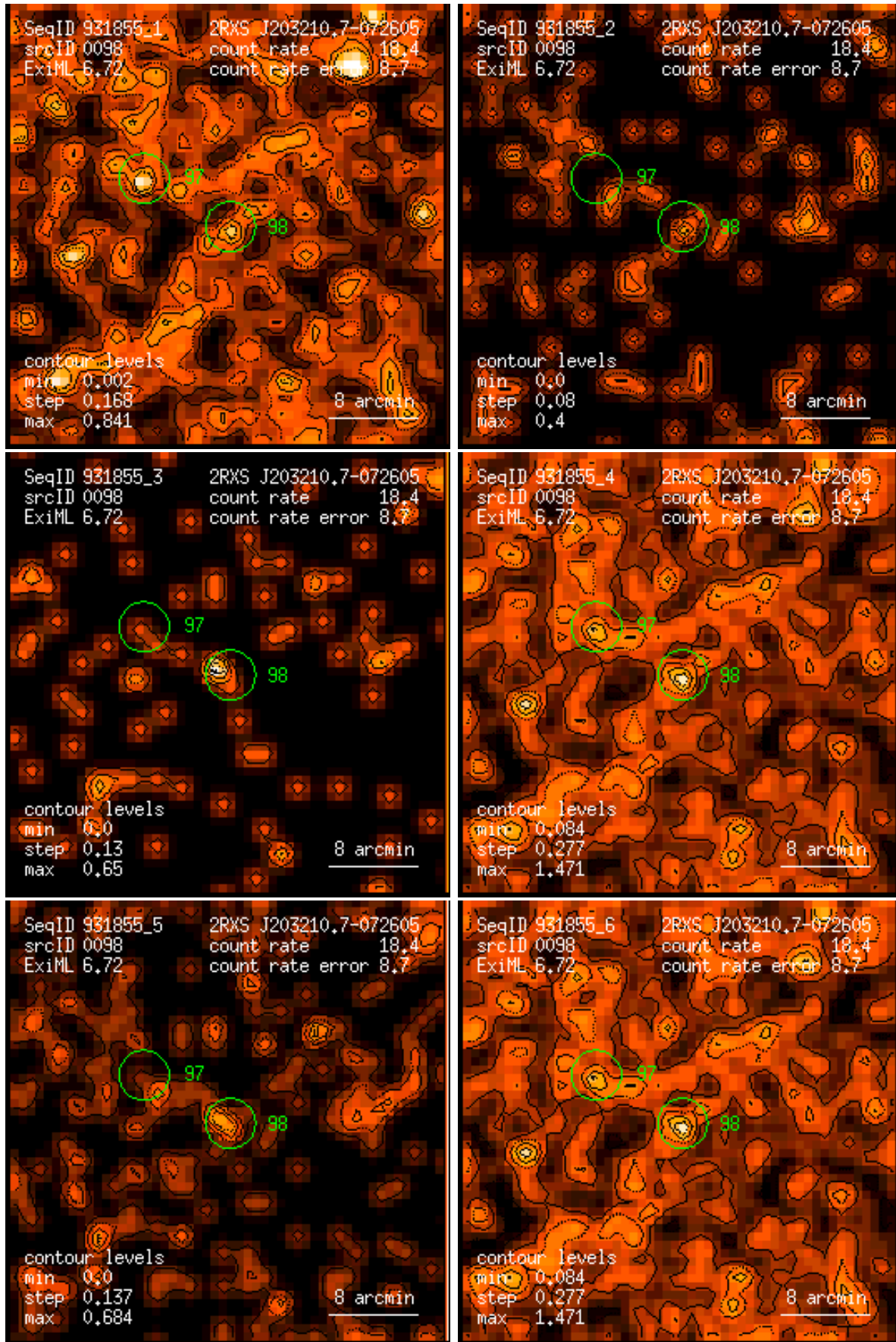
Figure 98: RASS 931855: detection 0098: band rate images, Gaussian filter: (1) PSPC channels 11 – 41, (2) 52 – 90, (3) 91 – 201, (4) 11 – 235, (5) 52 – 201, (6) 11 – 201. Broad band rates in counts/ks. Band rate contour levels in counts/ks/arcmin 2 .
