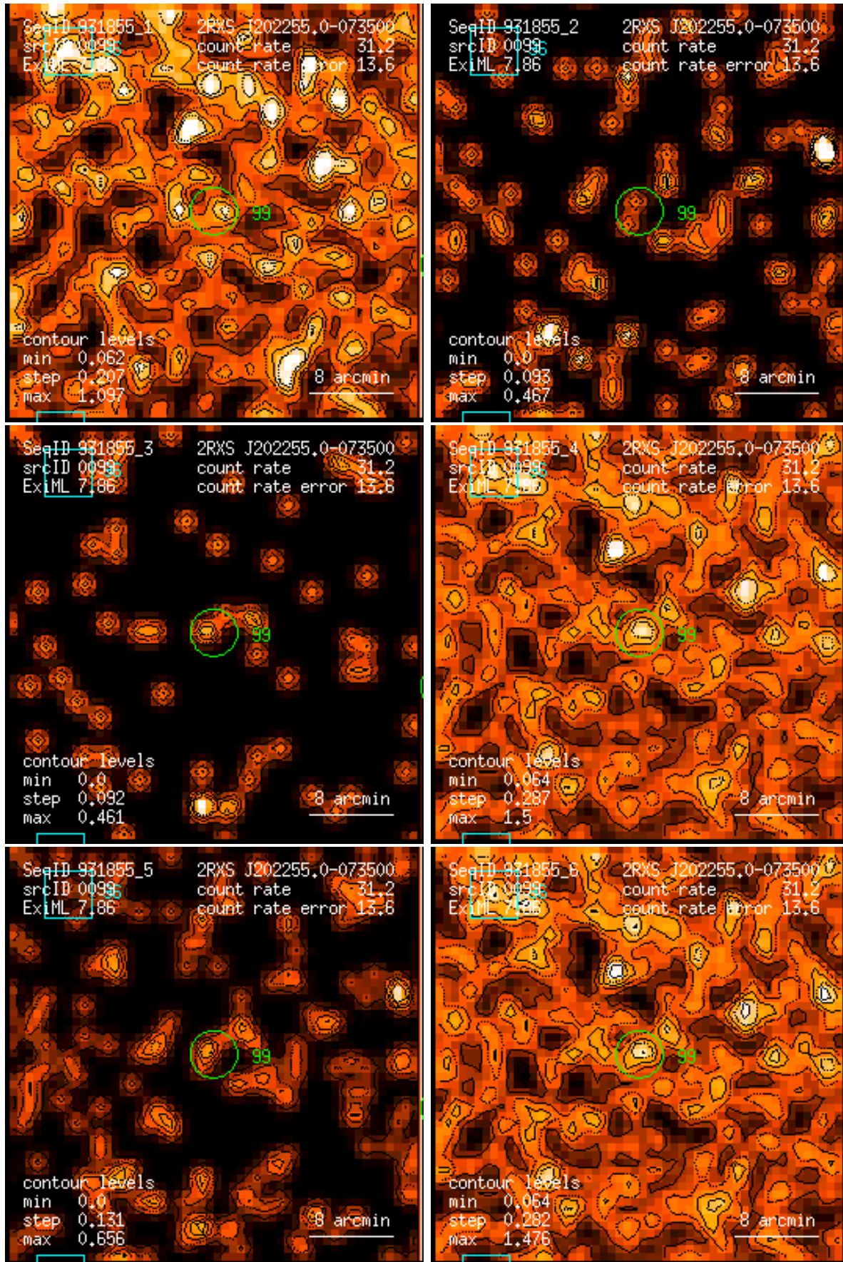
Figure 99: RASS 931855: detection 0099: band rate images, Gaussian filter: (1) PSPC channels 11 – 41, (2) 52 – 90, (3) 91 – 201, (4) 11 – 235, (5) 52 – 201, (6) 11 – 201. Broad band rates in counts/ks. Band rate contour levels in counts/ks/arcmin 2 .
