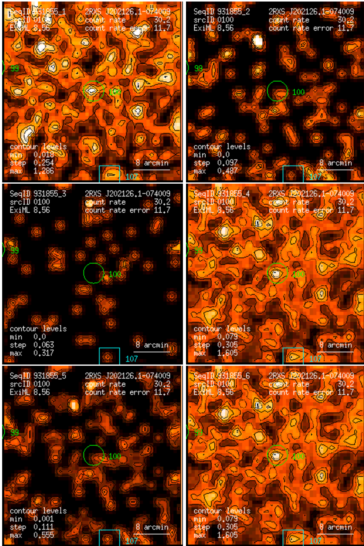
Figure 100: RASS 931855: detection 0100: band rate images, Gaussian filter: (1) PSPC channels 11 – 41, (2) 52 – 90, (3) 91 – 201, (4) 11 – 235, (5) 52 – 201, (6) 11 – 201. Broad band rates in counts/ks. Band rate contour levels in counts/ks/arcmin 2 .
