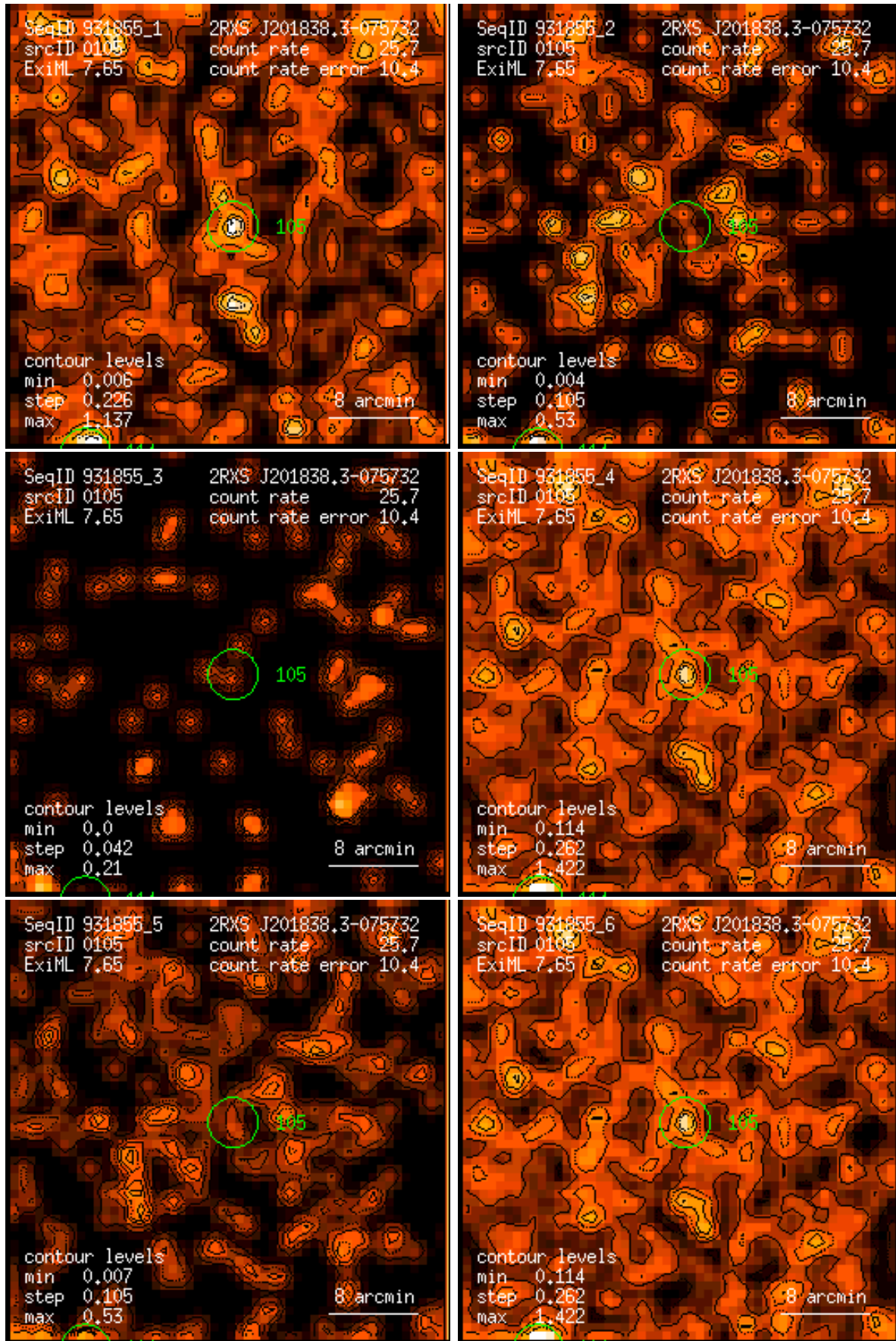
Figure 105: RASS 931855: detection 0105: band rate images, Gaussian filter: (1) PSPC channels 11 – 41, (2) 52 – 90, (3) 91 – 201, (4) 11 – 235, (5) 52 – 201, (6) 11 – 201. Broad band rates in counts/ks. Band rate contour levels in counts/ks/arcmin 2 .
