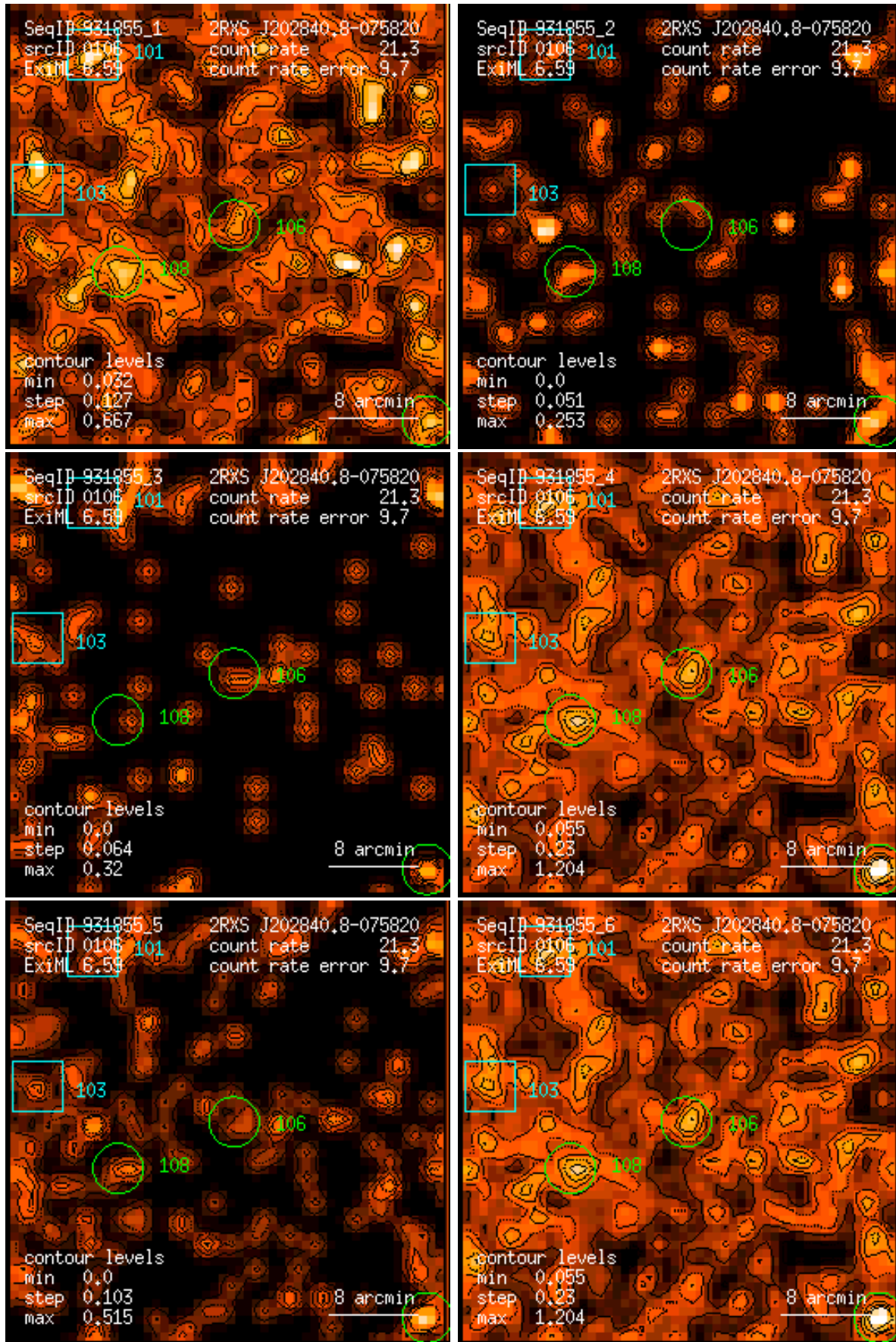
Figure 106: RASS 931855: detection 0106: band rate images, Gaussian filter: (1) PSPC channels 11 – 41, (2) 52 – 90, (3) 91 – 201, (4) 11 – 235, (5) 52 – 201, (6) 11 – 201. Broad band rates in counts/ks. Band rate contour levels in counts/ks/arcmin 2 .
