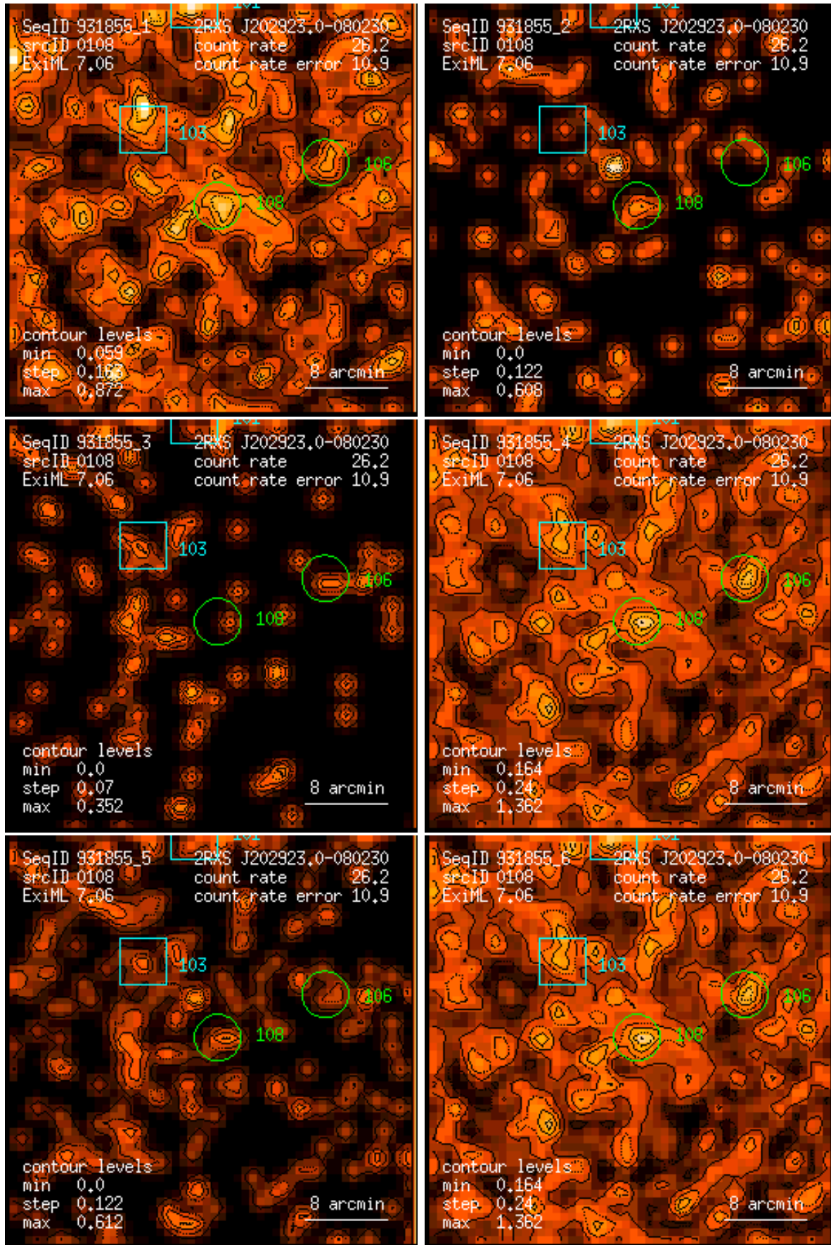
Figure 108: RASS 931855: detection 0108: band rate images, Gaussian filter: (1) PSPC channels 11 – 41, (2) 52 – 90, (3) 91 – 201, (4) 11 – 235, (5) 52 – 201, (6) 11 – 201. Broad band rates in counts/ks. Band rate contour levels in counts/ks/arcmin 2 .
