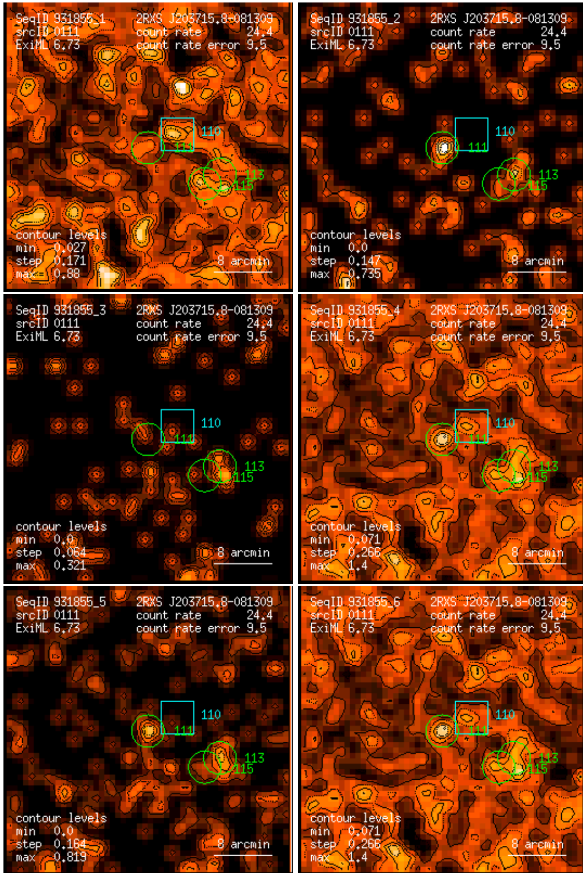
Figure 111: RASS 931855: detection 0111: band rate images, Gaussian filter: (1) PSPC channels 11 – 41, (2) 52 – 90, (3) 91 – 201, (4) 11 – 235, (5) 52 – 201, (6) 11 – 201. Broad band rates in counts/ks. Band rate contour levels in counts/ks/arcmin 2 .
