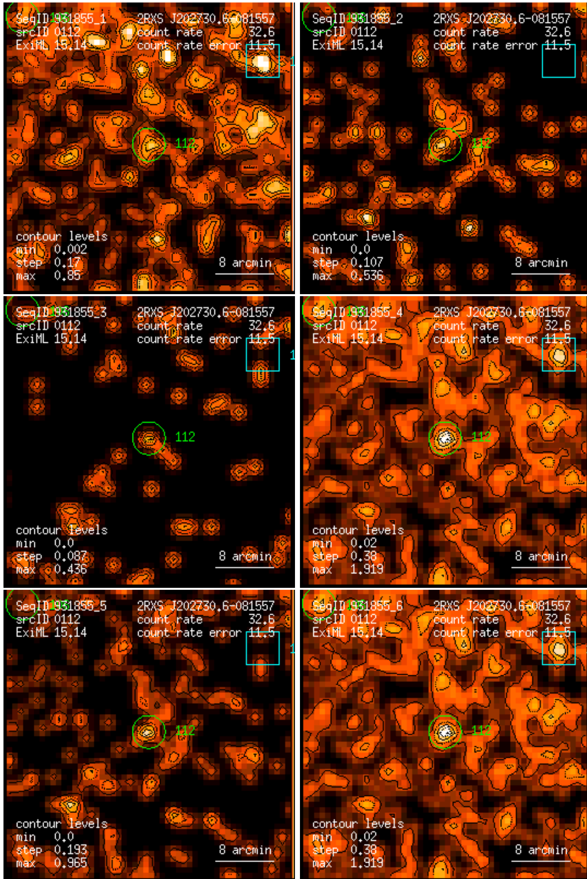
Figure 112: RASS 931855: detection 0112: band rate images, Gaussian filter: (1) PSPC channels 11 – 41, (2) 52 – 90, (3) 91 – 201, (4) 11 – 235, (5) 52 – 201, (6) 11 – 201. Broad band rates in counts/ks. Band rate contour levels in counts/ks/arcmin 2 .
