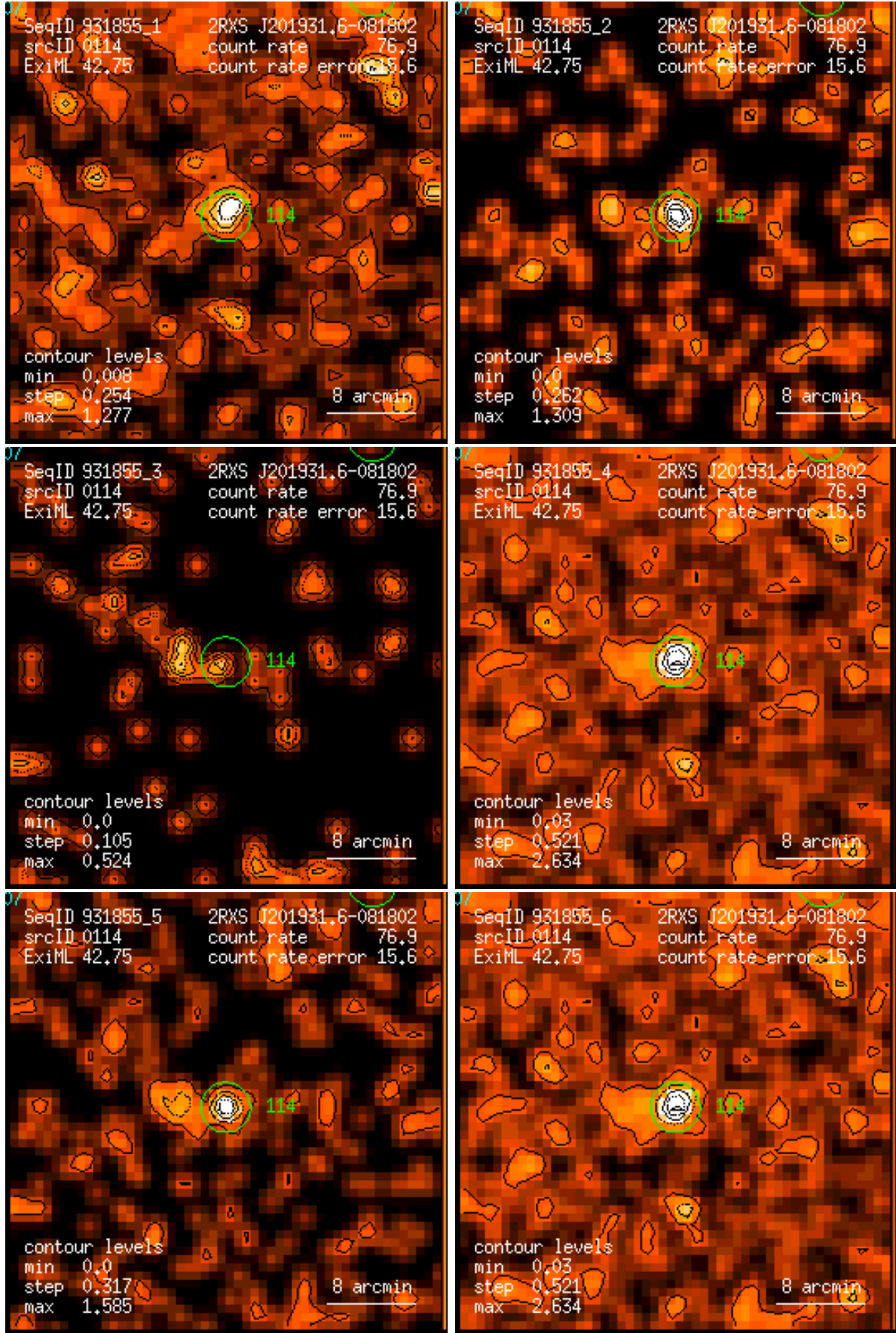
Figure 114: RASS 931855: detection 0114: band rate images, Gaussian filter: (1) PSPC channels 11 – 41, (2) 52 – 90, (3) 91 – 201, (4) 11 – 235, (5) 52 – 201, (6) 11 – 201. Broad band rates in counts/ks. Band rate contour levels in counts/ks/arcmin 2 .
