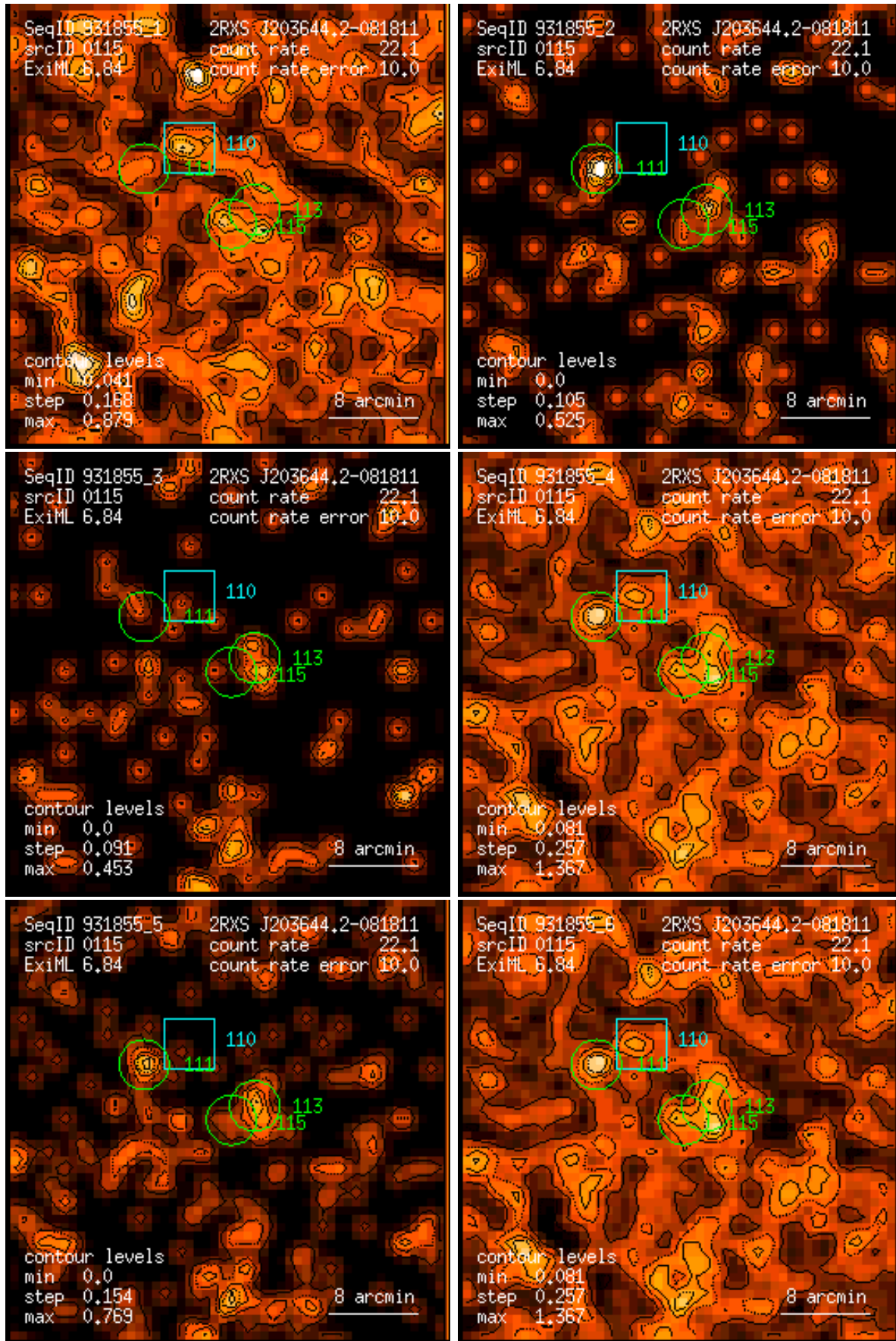
Figure 115: RASS 931855: detection 0115: band rate images, Gaussian filter: (1) PSPC channels 11 – 41, (2) 52 – 90, (3) 91 – 201, (4) 11 – 235, (5) 52 – 201, (6) 11 – 201. Broad band rates in counts/ks. Band rate contour levels in counts/ks/arcmin 2 .
