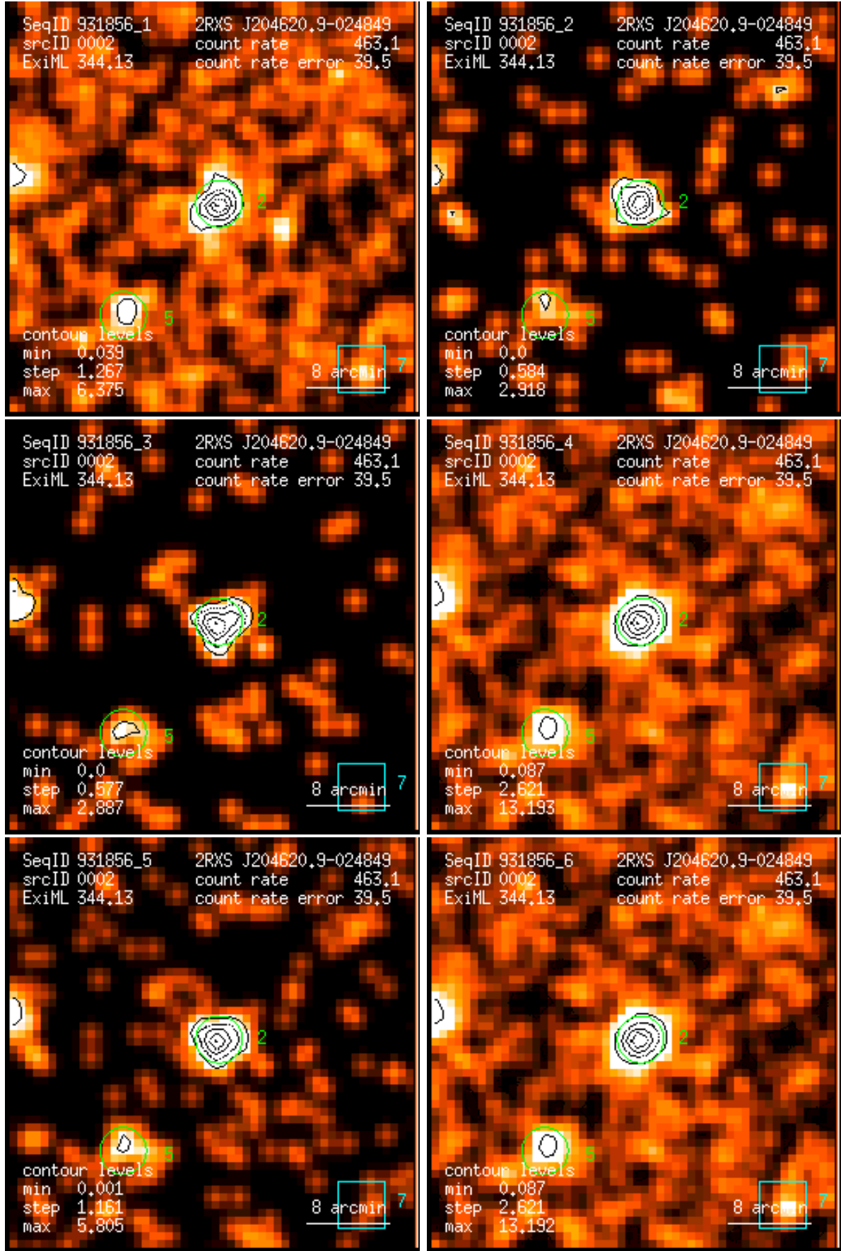
Figure 2: RASS 931856: detection 0002: band rate images, Gaussian filter: (1) PSPC channels 11 – 41, (2) 52 – 90, (3) 91 – 201, (4) 11 – 235, (5) 52 – 201, (6) 11 – 201. Broad band rates in counts/ks. Band rate contour levels in counts/ks/arcmin 2 .
