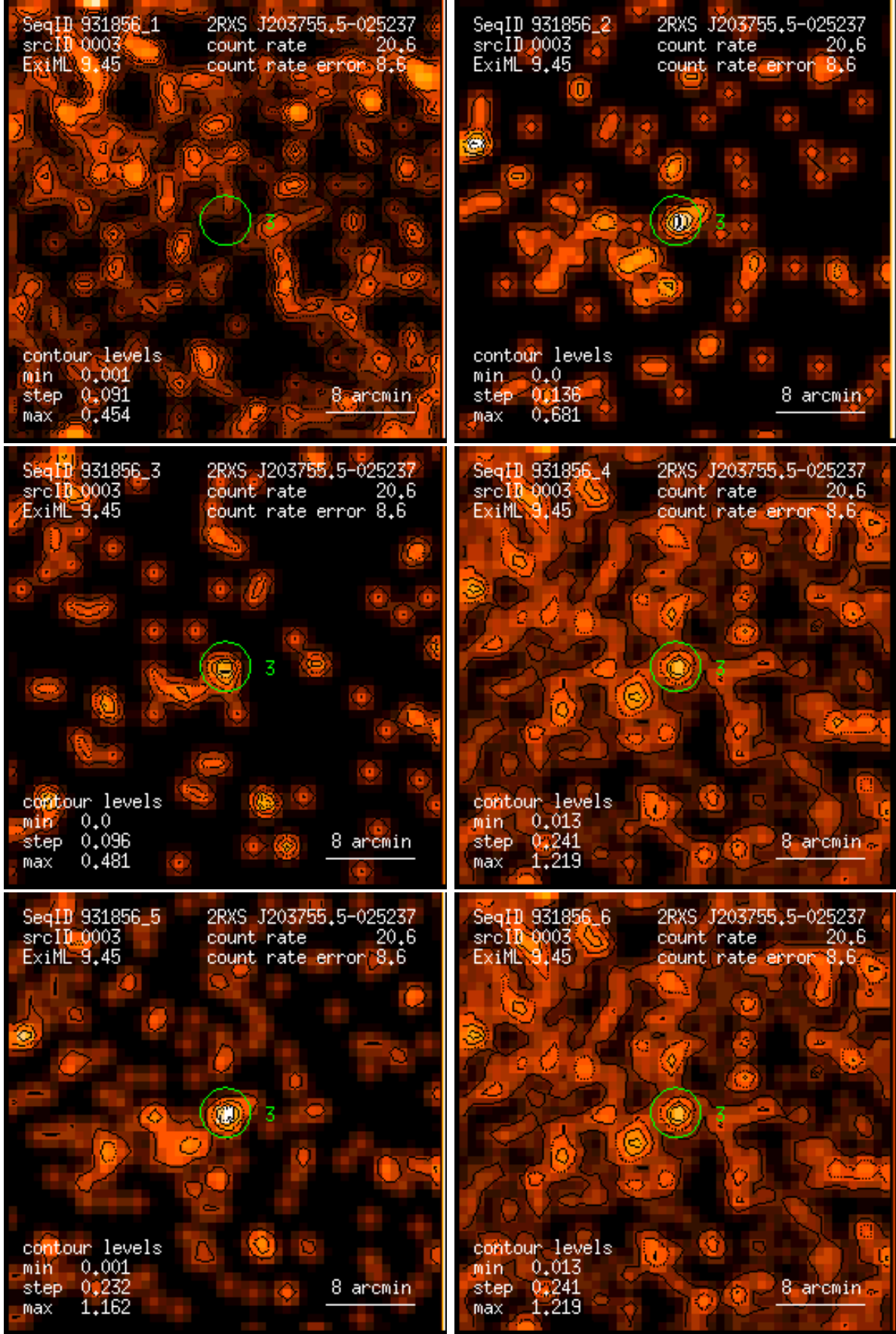
Figure 3: RASS 931856: detection 0003: band rate images, Gaussian filter: (1) PSPC channels 11 – 41, (2) 52 – 90, (3) 91 – 201, (4) 11 – 235, (5) 52 – 201, (6) 11 – 201. Broad band rates in counts/ks. Band rate contour levels in counts/ks/arcmin 2 .
