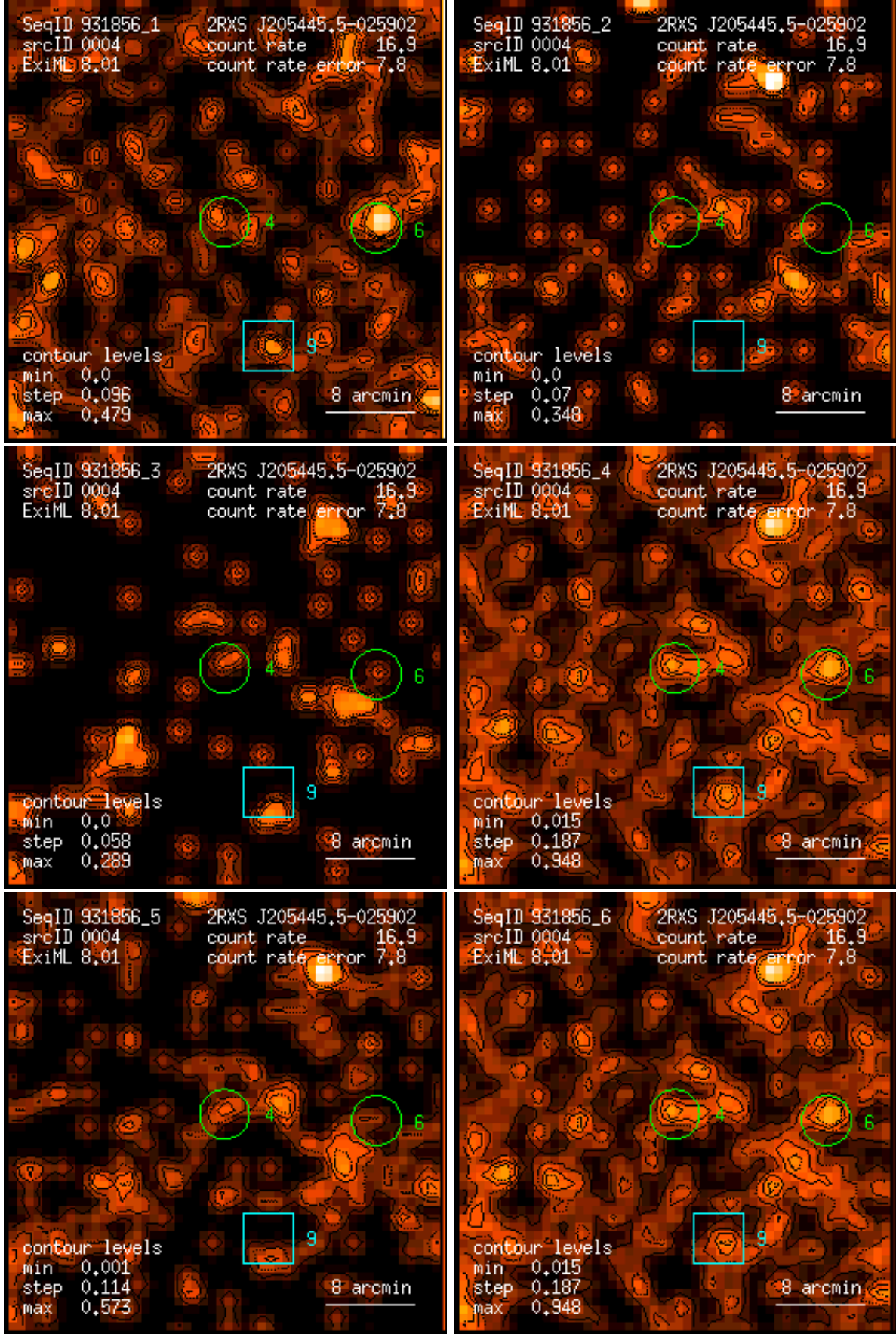
Figure 4: RASS 931856: detection 0004: band rate images, Gaussian filter: (1) PSPC channels 11 – 41, (2) 52 – 90, (3) 91 – 201, (4) 11 – 235, (5) 52 – 201, (6) 11 – 201. Broad band rates in counts/ks. Band rate contour levels in counts/ks/arcmin 2 .
