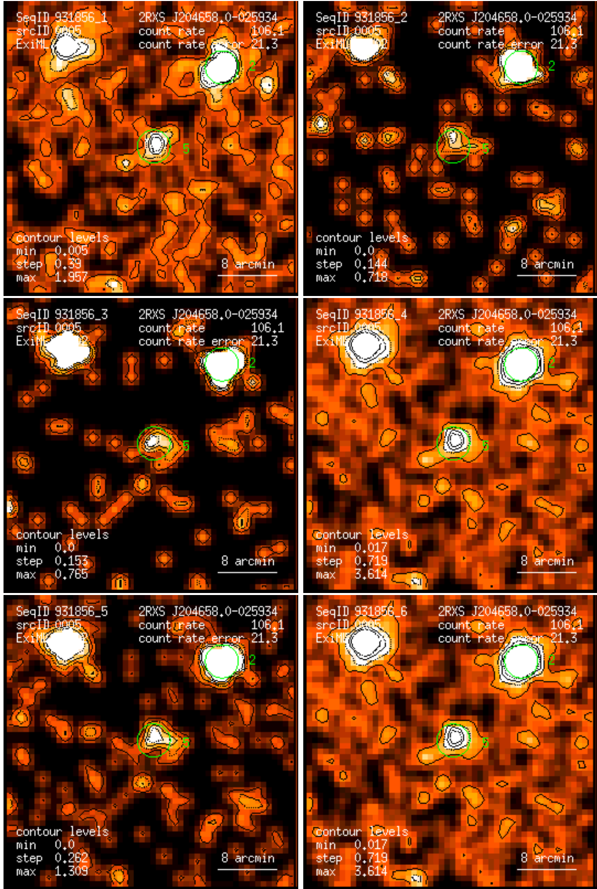
Figure 5: RASS 931856: detection 0005: band rate images, Gaussian filter: (1) PSPC channels 11 – 41, (2) 52 – 90, (3) 91 – 201, (4) 11 – 235, (5) 52 – 201, (6) 11 – 201. Broad band rates in counts/ks. Band rate contour levels in counts/ks/arcmin 2 .
