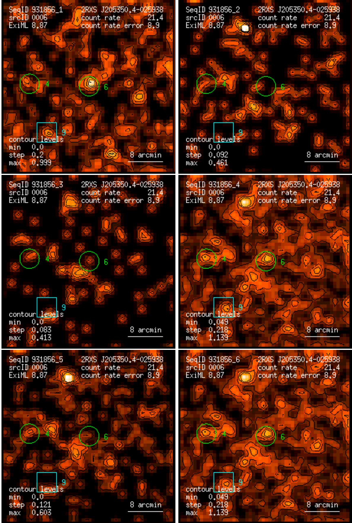
Figure 6: RASS 931856: detection 0006: band rate images, Gaussian filter: (1) PSPC channels 11 – 41, (2) 52 – 90, (3) 91 – 201, (4) 11 – 235, (5) 52 – 201, (6) 11 – 201. Broad band rates in counts/ks. Band rate contour levels in counts/ks/arcmin 2 .
