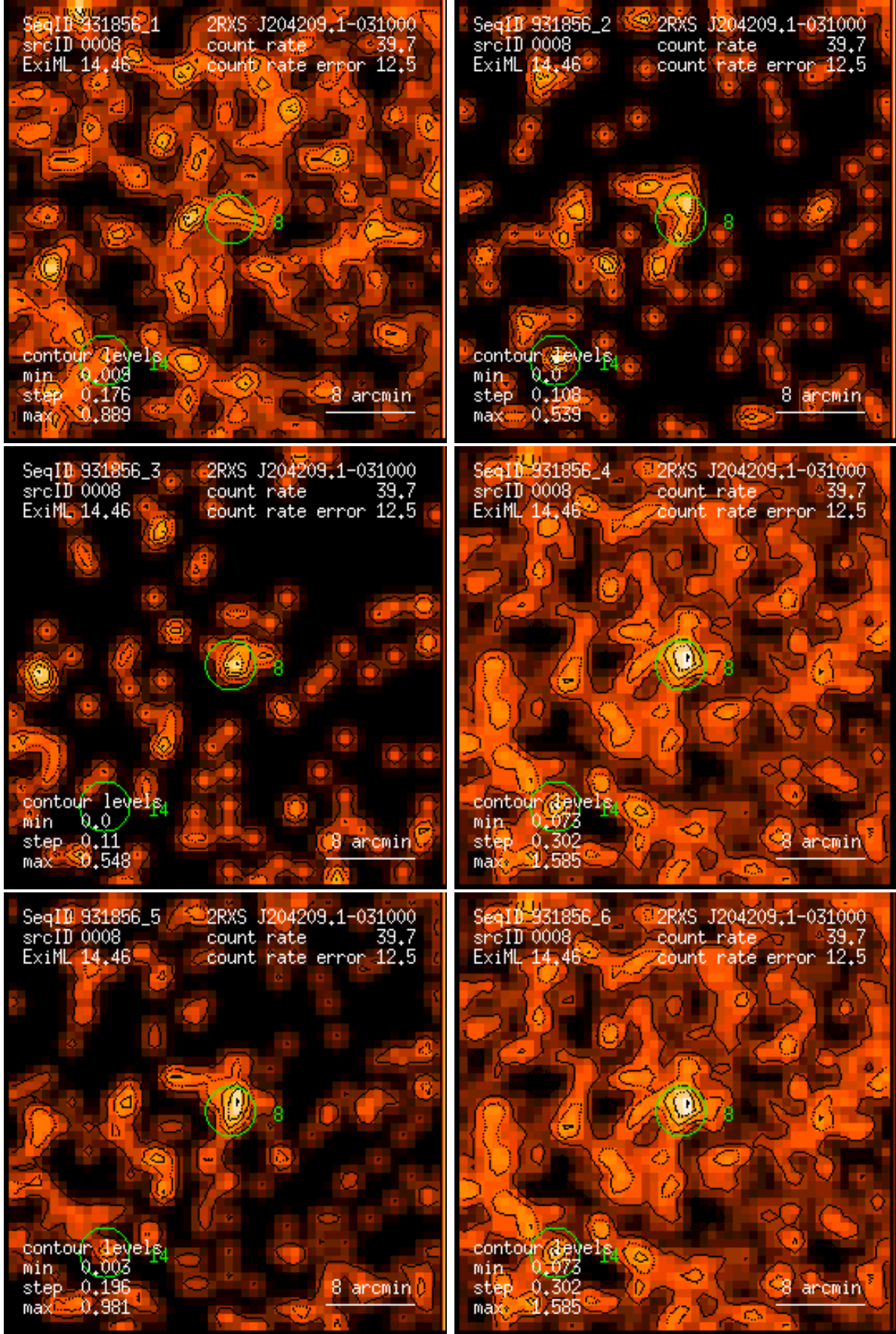
Figure 8: RASS 931856: detection 0008: band rate images, Gaussian filter: (1) PSPC channels 11 – 41, (2) 52 – 90, (3) 91 – 201, (4) 11 – 235, (5) 52 – 201, (6) 11 – 201. Broad band rates in counts/ks. Band rate contour levels in counts/ks/arcmin 2 .
