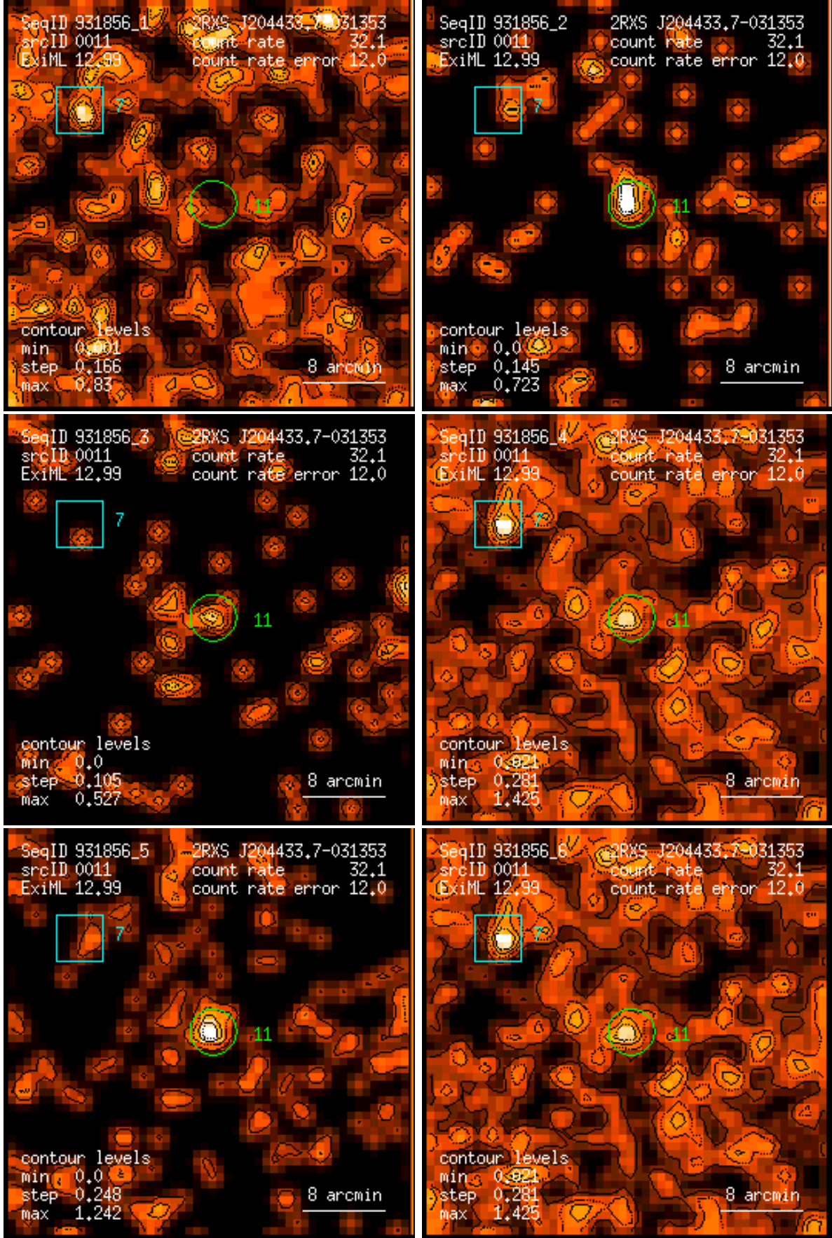
Figure 11: RASS 931856: detection 0011: band rate images, Gaussian filter: (1) PSPC channels 11 – 41, (2) 52 – 90, (3) 91 – 201, (4) 11 – 235, (5) 52 – 201, (6) 11 – 201. Broad band rates in counts/ks. Band rate contour levels in counts/ks/arcmin 2 .
