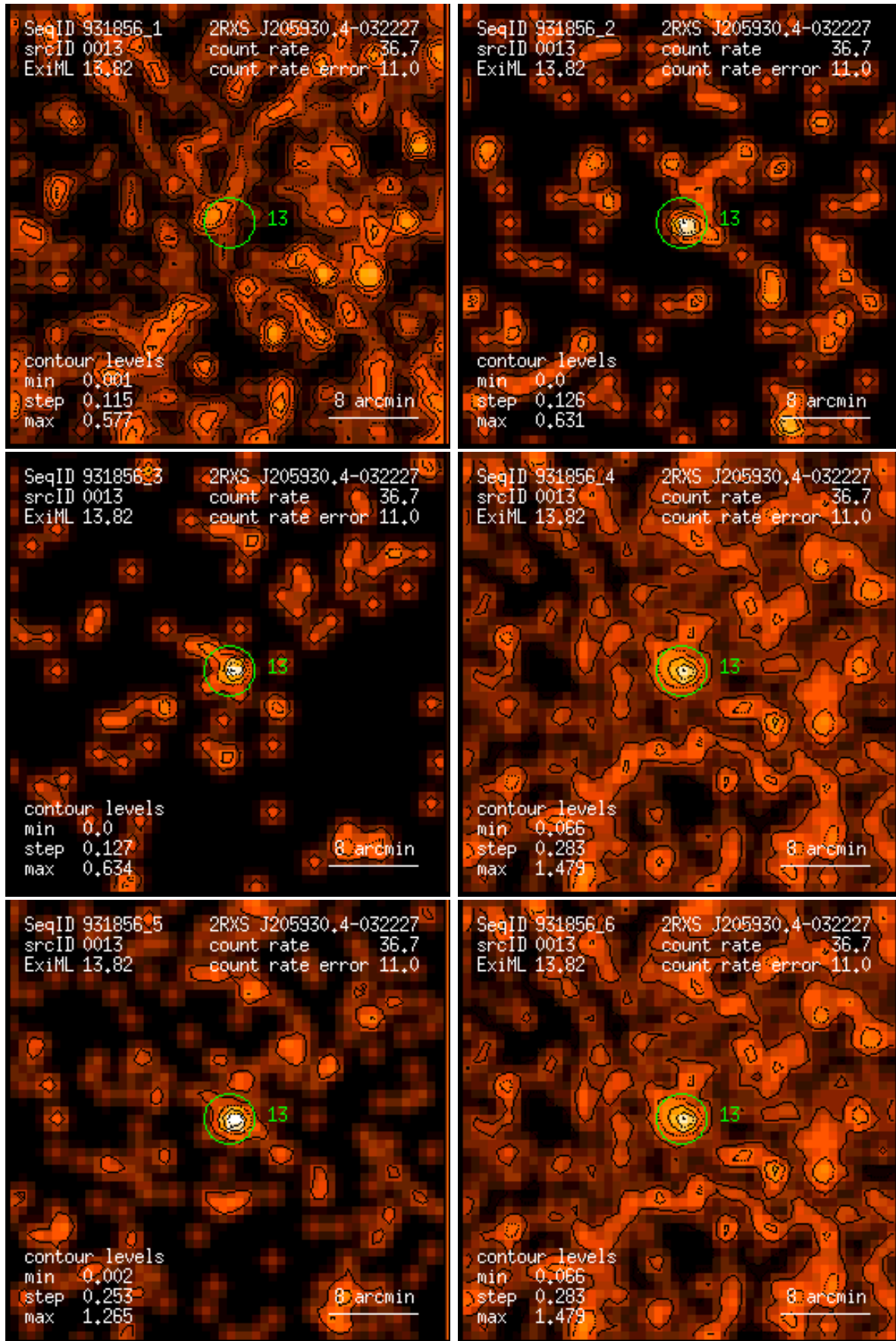
Figure 13: RASS 931856: detection 0013: band rate images, Gaussian filter: (1) PSPC channels 11 – 41, (2) 52 – 90, (3) 91 – 201, (4) 11 – 235, (5) 52 – 201, (6) 11 – 201. Broad band rates in counts/ks. Band rate contour levels in counts/ks/arcmin 2 .
