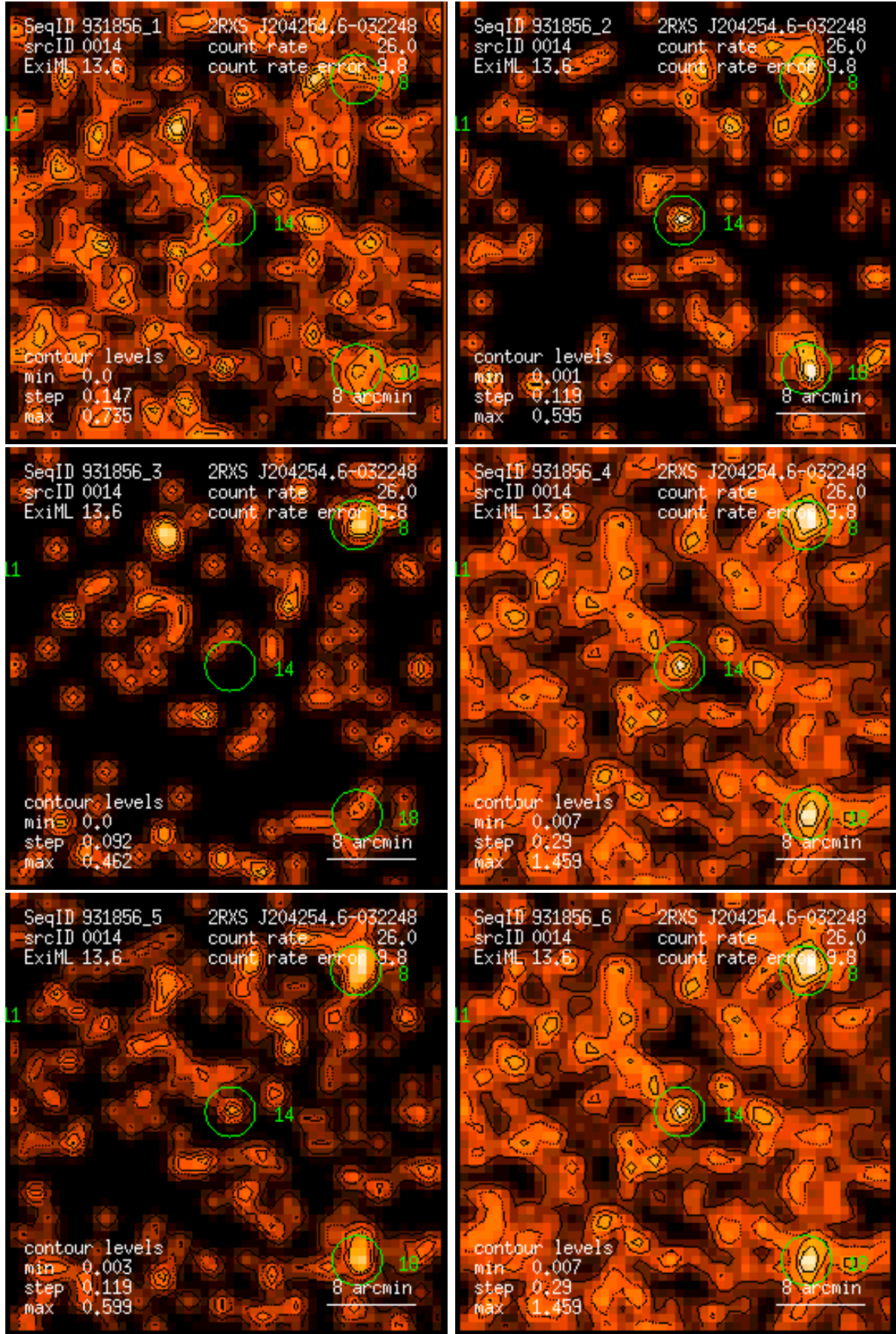
Figure 14: RASS 931856: detection 0014: band rate images, Gaussian filter: (1) PSPC channels 11 – 41, (2) 52 – 90, (3) 91 – 201, (4) 11 – 235, (5) 52 – 201, (6) 11 – 201. Broad band rates in counts/ks. Band rate contour levels in counts/ks/arcmin 2 .
