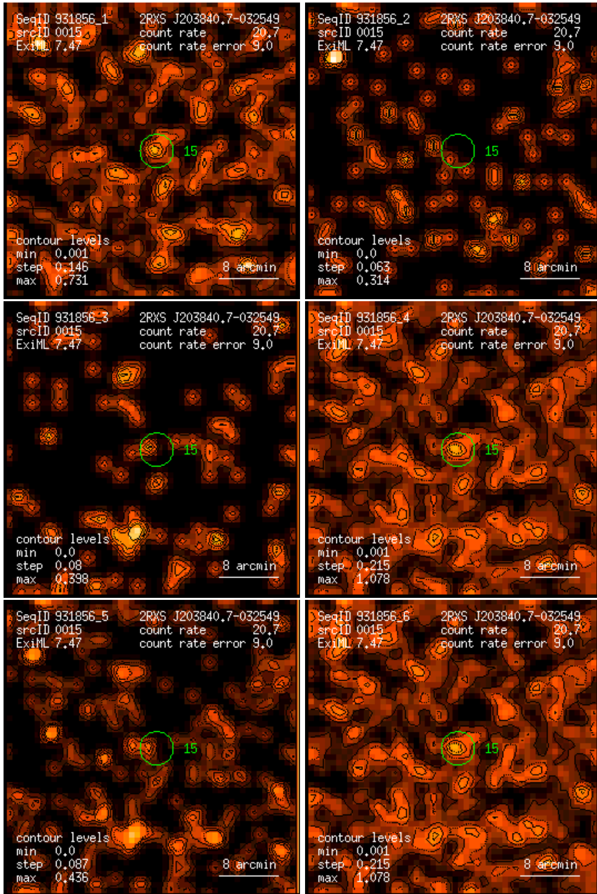
Figure 15: RASS 931856: detection 0015: band rate images, Gaussian filter: (1) PSPC channels 11 – 41, (2) 52 – 90, (3) 91 – 201, (4) 11 – 235, (5) 52 – 201, (6) 11 – 201. Broad band rates in counts/ks. Band rate contour levels in counts/ks/arcmin 2 .
