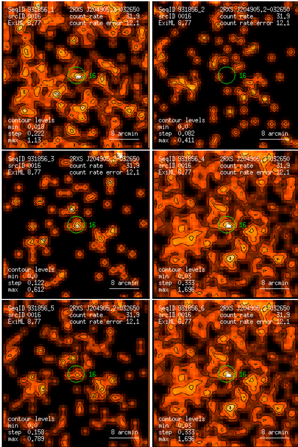
Figure 16: RASS 931856: detection 0016: band rate images, Gaussian filter: (1) PSPPC channels 11 – 41, (2) 52 – 90, (3) 91 – 201, (4) 11 – 235, (5) 52 – 201, (6) 11 – 201. Broad band rates in counts/ks. Band rate contour levels in counts/ks/arcmin 2 .
