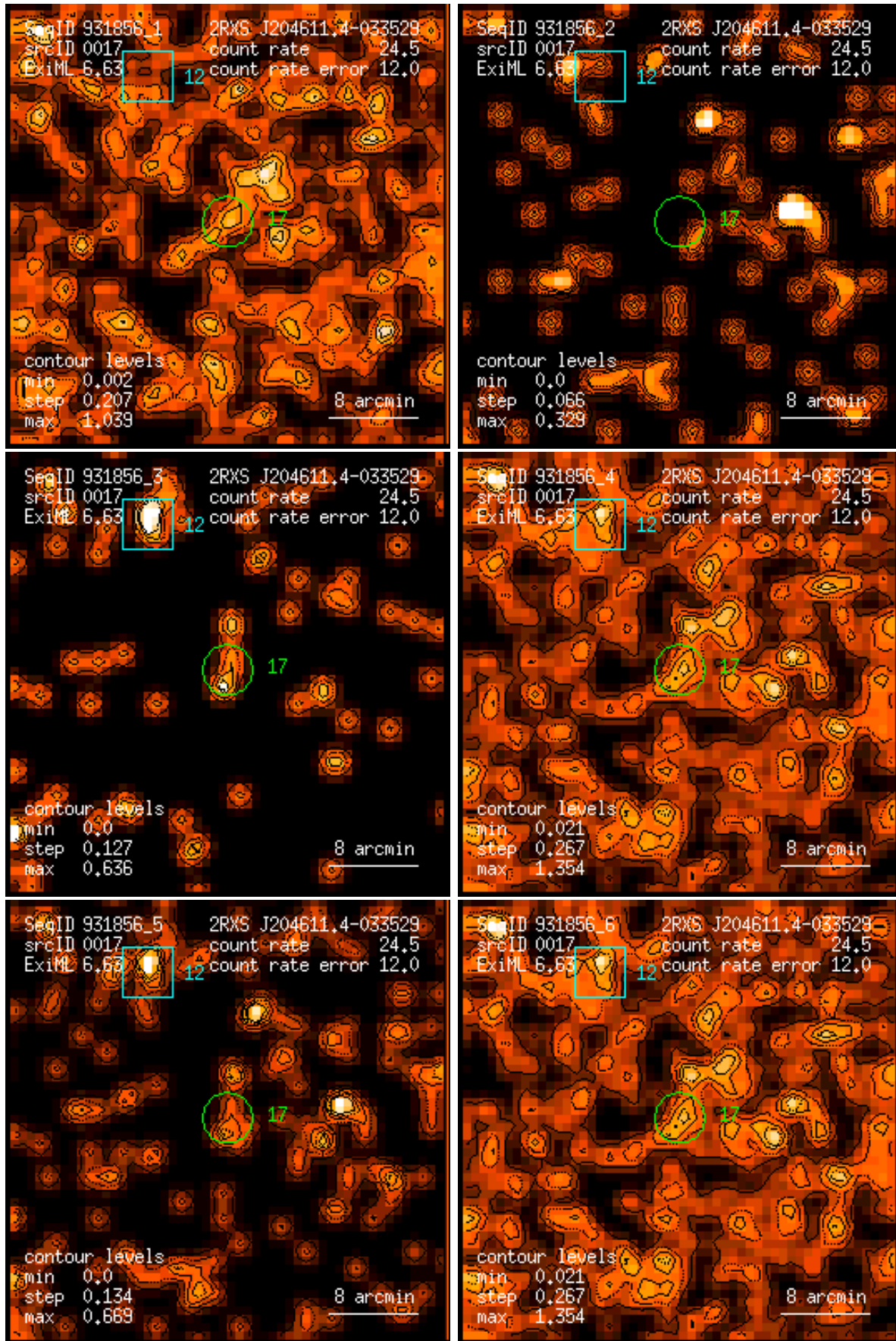
Figure 17: RASS 931856: detection 0017: band rate images, Gaussian filter: (1) PSPC channels 11 – 41, (2) 52 – 90, (3) 91 – 201, (4) 11 – 235, (5) 52 – 201, (6) 11 – 201. Broad band rates in counts/ks. Band rate contour levels in counts/ks/arcmin 2 .
