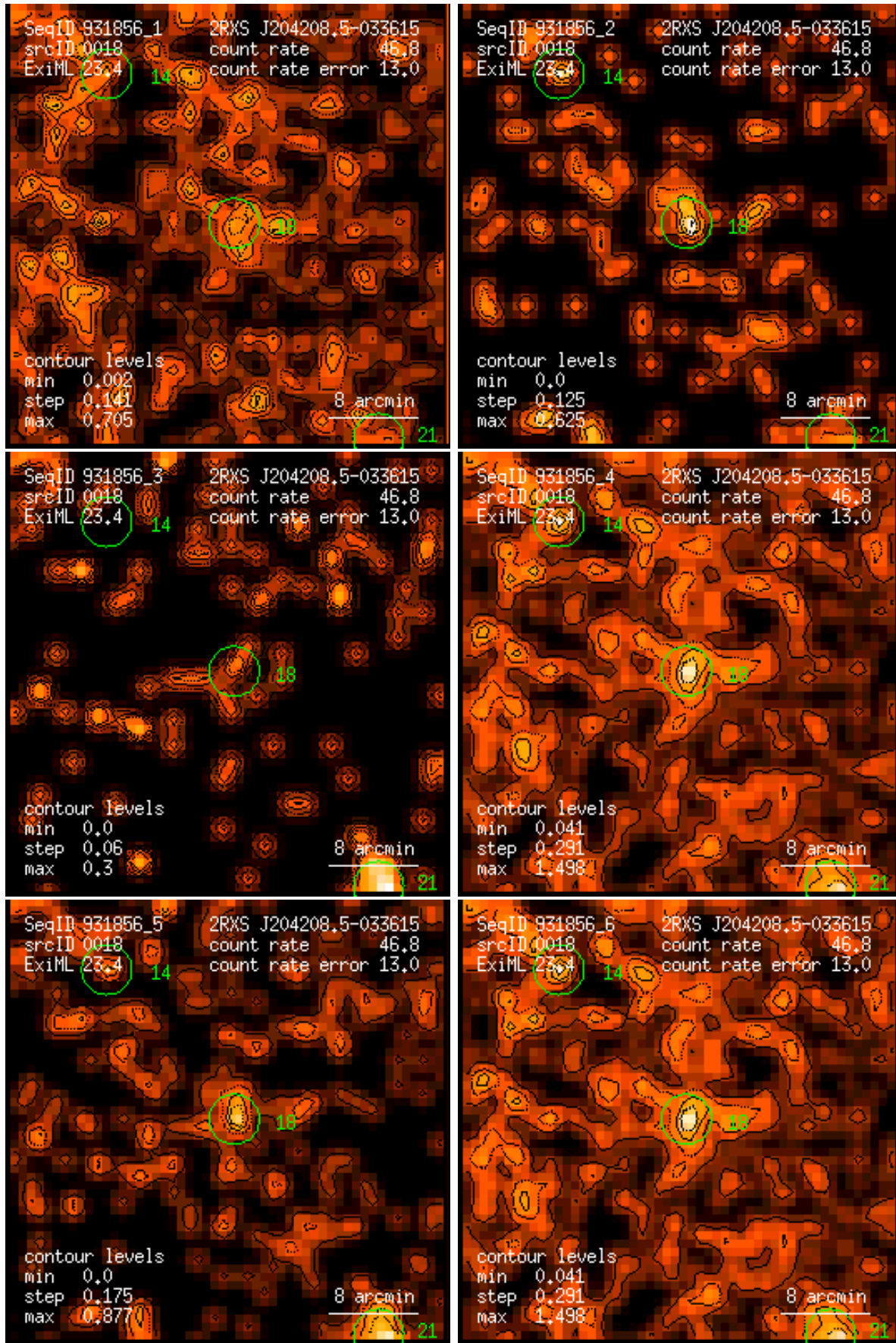
Figure 18: RASS 931856: detection 0018: band rate images, Gaussian filter: (1) PSPC channels 11 – 41, (2) 52 – 90, (3) 91 – 201, (4) 11 – 235, (5) 52 – 201, (6) 11 – 201. Broad band rates in counts/ks. Band rate contour levels in counts/ks/arcmin 2 .
