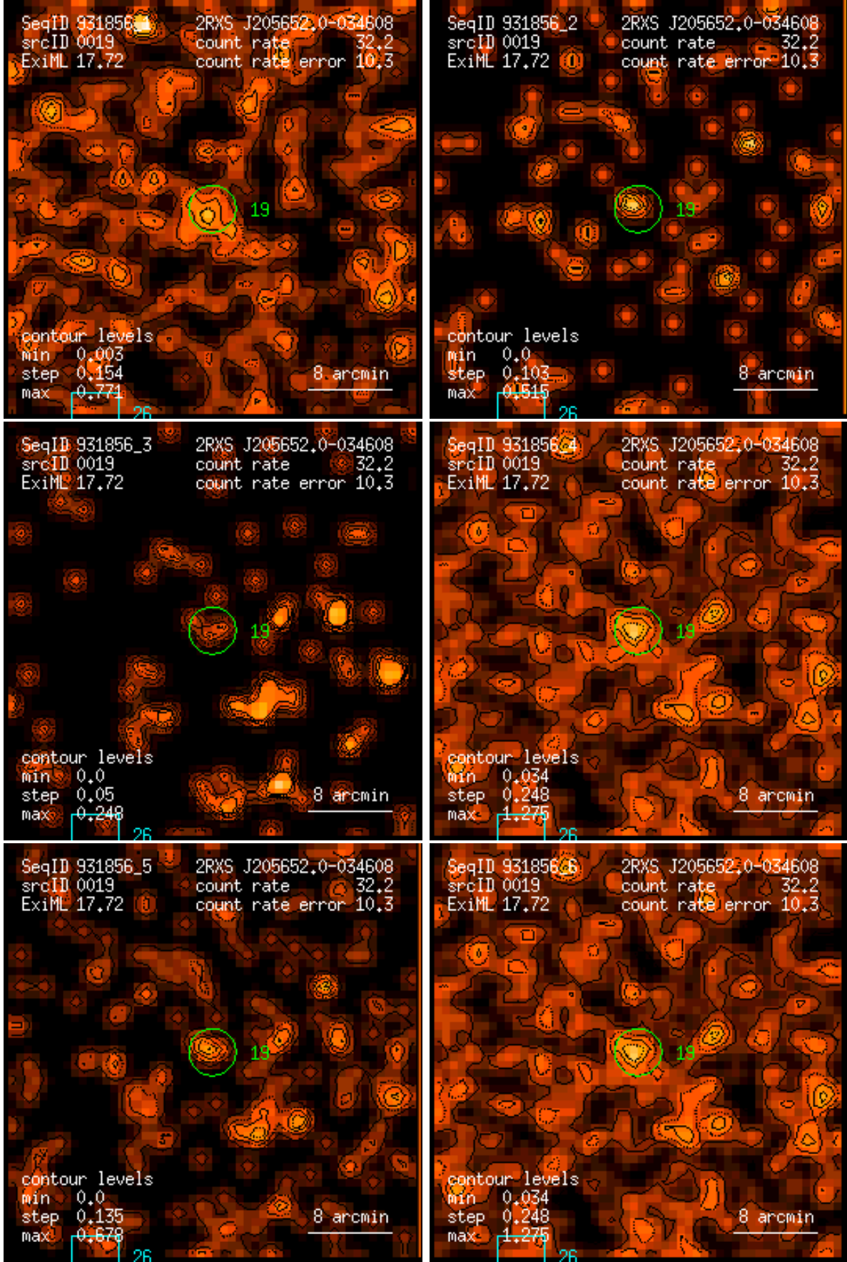
Figure 19: RASS 931856: detection 0019: band rate images, Gaussian filter: (1) PSPC channels 11 – 41, (2) 52 – 90, (3) 91 – 201, (4) 11 – 235, (5) 52 – 201, (6) 11 – 201. Broad band rates in counts/ks. Band rate contour levels in counts/ks/arcmin 2 .
