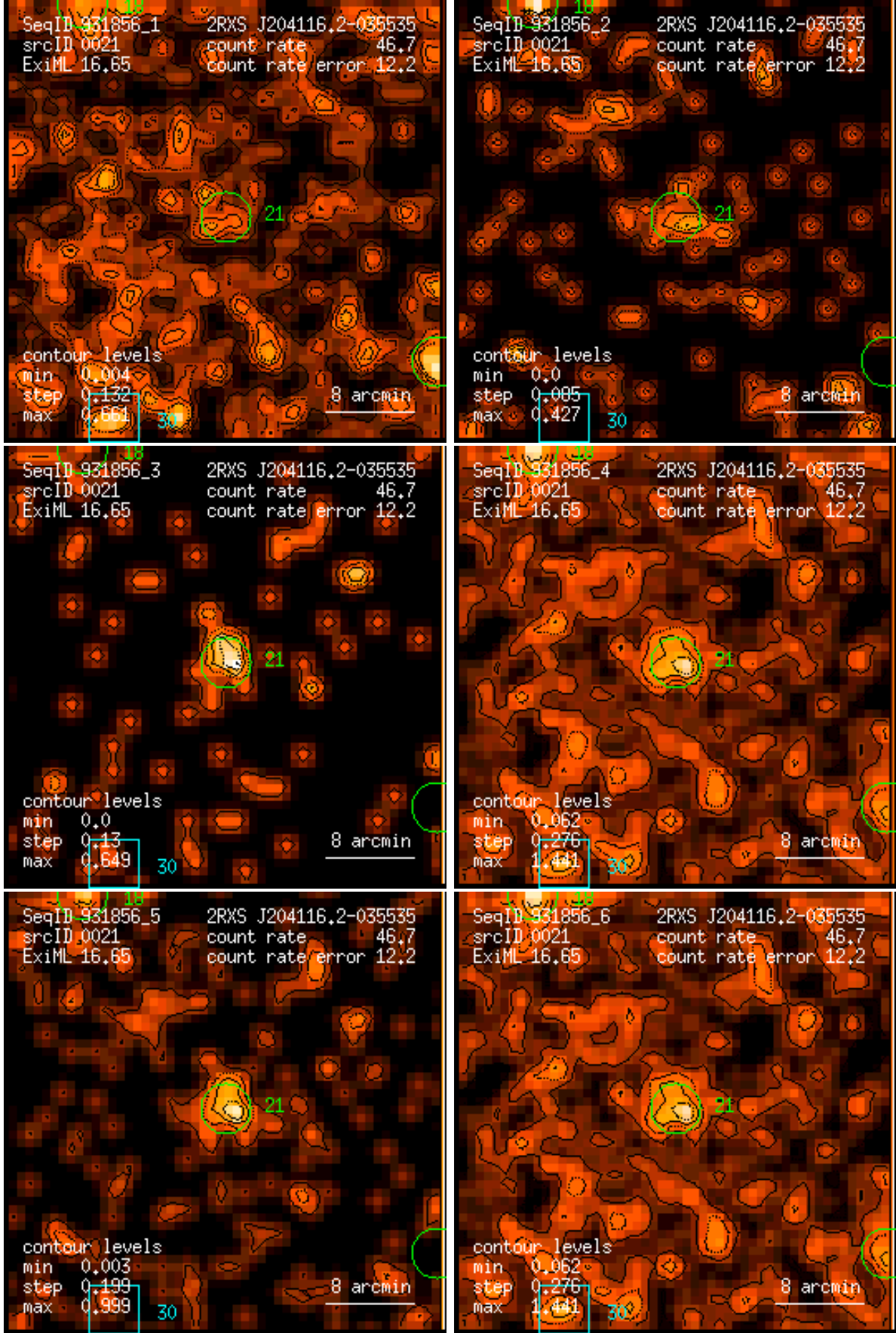
Figure 21: RASS 931856: detection 0021: band rate images, Gaussian filter: (1) PSPC channels 11 – 41, (2) 52 – 90, (3) 91 – 201, (4) 11 – 235, (5) 52 – 201, (6) 11 – 201. Broad band rates in counts/ks. Band rate contour levels in counts/ks/arcmin 2 .
