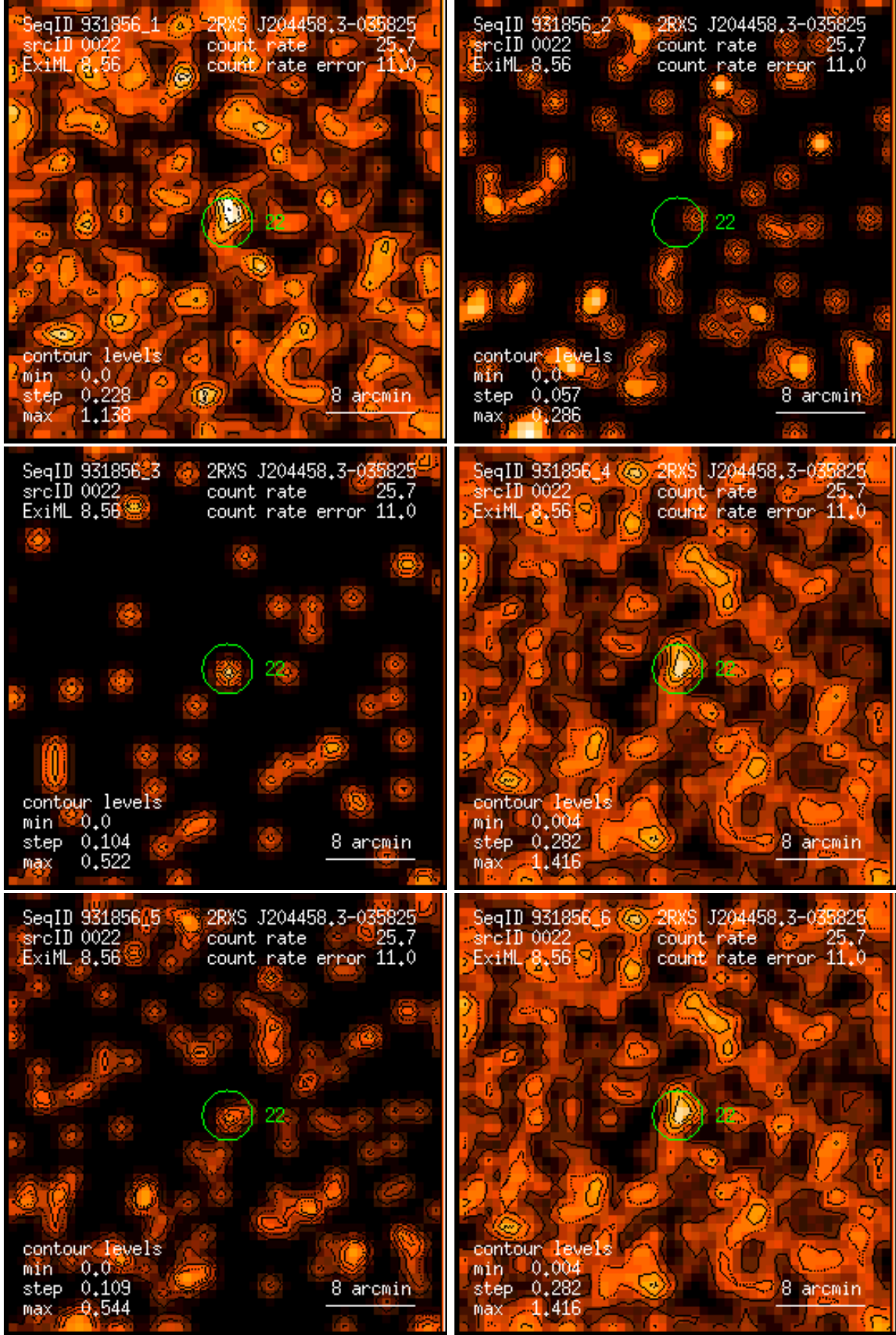
Figure 22: RASS 931856: detection 0022: band rate images, Gaussian filter: (1) PSPC channels 11 – 41, (2) 52 – 90, (3) 91 – 201, (4) 11 – 235, (5) 52 – 201, (6) 11 – 201. Broad band rates in counts/ks. Band rate contour levels in counts/ks/arcmin 2 .
