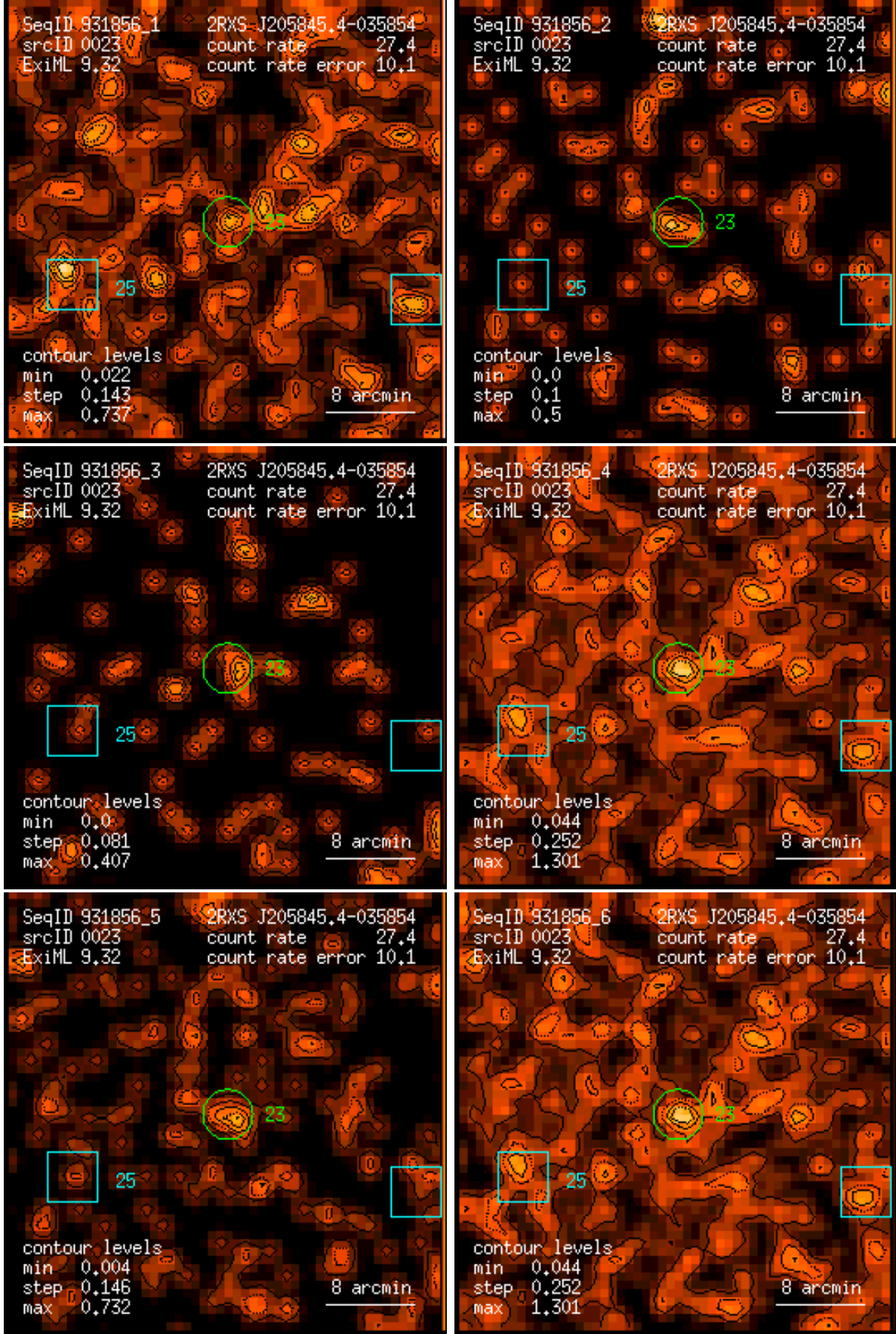
Figure 23: RASS 931856: detection 0023: band rate images, Gaussian filter: (1) PSPC channels 11 – 41, (2) 52 – 90, (3) 91 – 201, (4) 11 – 235, (5) 52 – 201, (6) 11 – 201. Broad band rates in counts/ks. Band rate contour levels in counts/ks/arcmin 2 .
