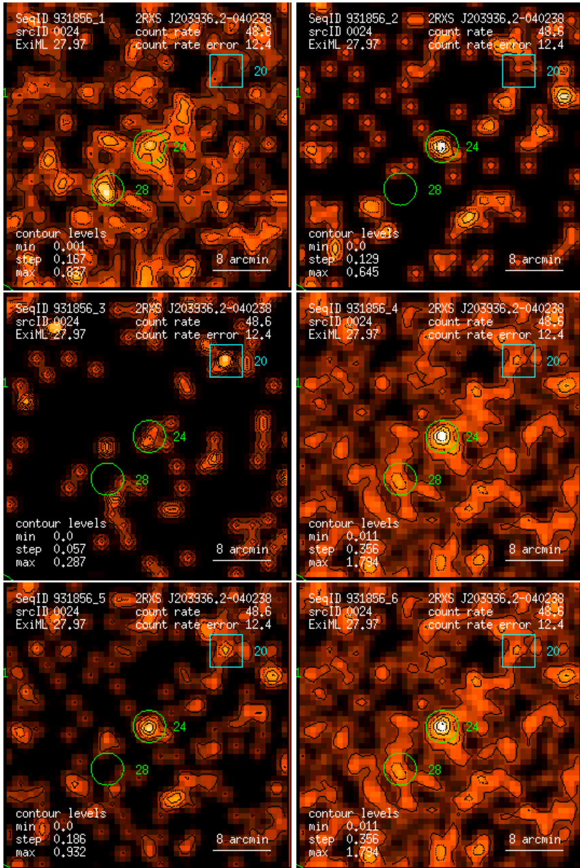
Figure 24: RASS 931856: detection 0024: band rate images, Gaussian filter: (1) PSPC channels 11 – 41, (2) 52 – 90, (3) 91 – 201, (4) 11 – 235, (5) 52 – 201, (6) 11 – 201. Broad band rates in counts/ks. Band rate contour levels in counts/ks/arcmin 2 .
