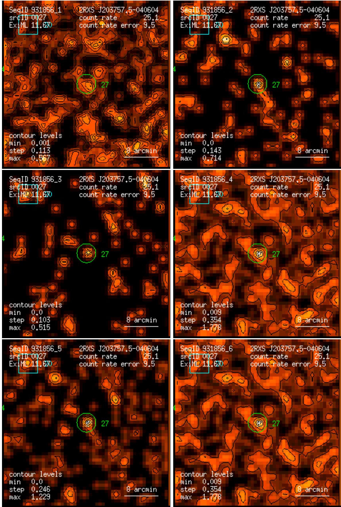
Figure 27: RASS 931856: detection 0027: band rate images, Gaussian filter: (1) PSPC channels 11 – 41, (2) 52 – 90, (3) 91 – 201, (4) 11 – 235, (5) 52 – 201, (6) 11 – 201. Broad band rates in counts/ks. Band rate contour levels in counts/ks/arcmin 2 .
