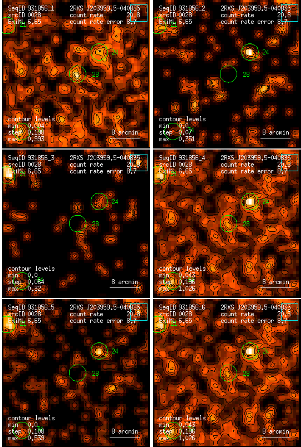
Figure 28: RASS 931856: detection 0028: band rate images, Gaussian filter: (1) PSPC channels 11 – 41, (2) 52 – 90, (3) 91 – 201, (4) 11 – 235, (5) 52 – 201, (6) 11 – 201. Broad band rates in counts/ks. Band rate contour levels in counts/ks/arcmin 2 .
