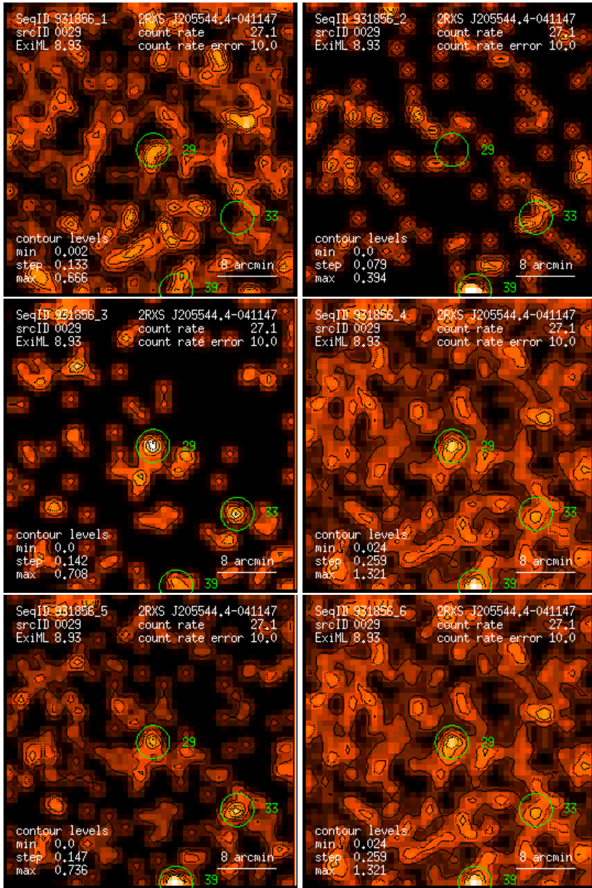
Figure 29: RASS 931856: detection 0029: band rate images, Gaussian filter: (1) PSPC channels 11 – 41, (2) 52 – 90, (3) 91 – 201, (4) 11 – 235, (5) 52 – 201, (6) 11 – 201. Broad band rates in counts/ks. Band rate contour levels in counts/ks/arcmin 2 .
