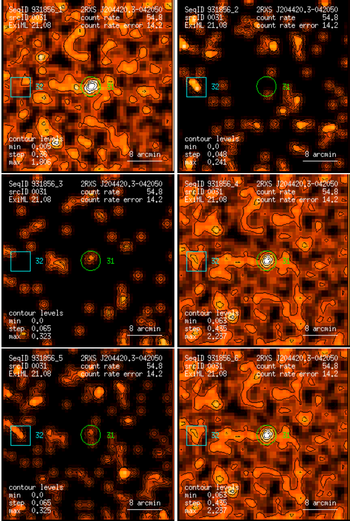
Figure 31: RASS 931856: detection 0031: band rate images, Gaussian filter: (1) PSPC channels 11 – 41, (2) 52 – 90, (3) 91 – 201, (4) 11 – 235, (5) 52 – 201, (6) 11 – 201. Broad band rates in counts/ks. Band rate contour levels in counts/ks/arcmin 2 .
