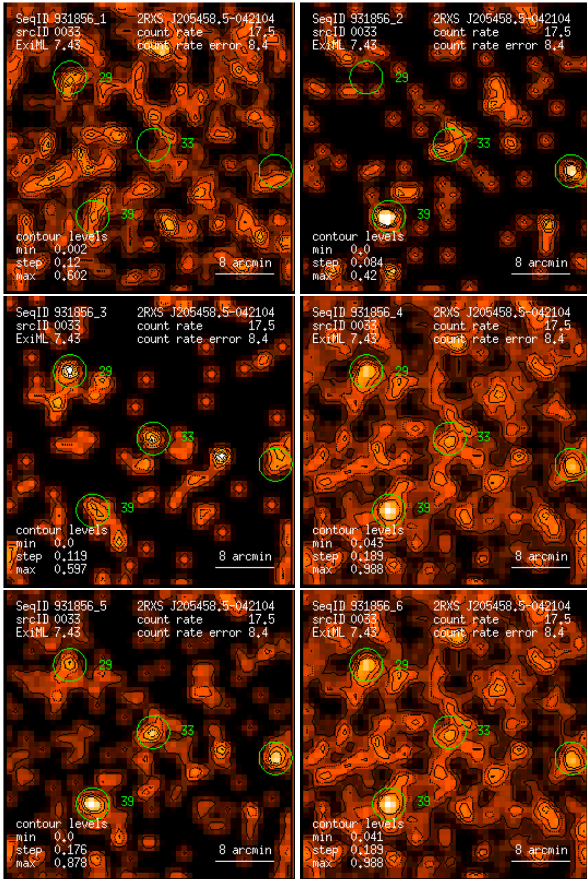
Figure 33: RASS 931856: detection 0033: band rate images, Gaussian filter: (1) PSPC channels 11 – 41, (2) 52 – 90, (3) 91 – 201, (4) 11 – 235, (5) 52 – 201, (6) 11 – 201. Broad band rates in counts/ks. Band rate contour levels in counts/ks/arcmin 2 .
