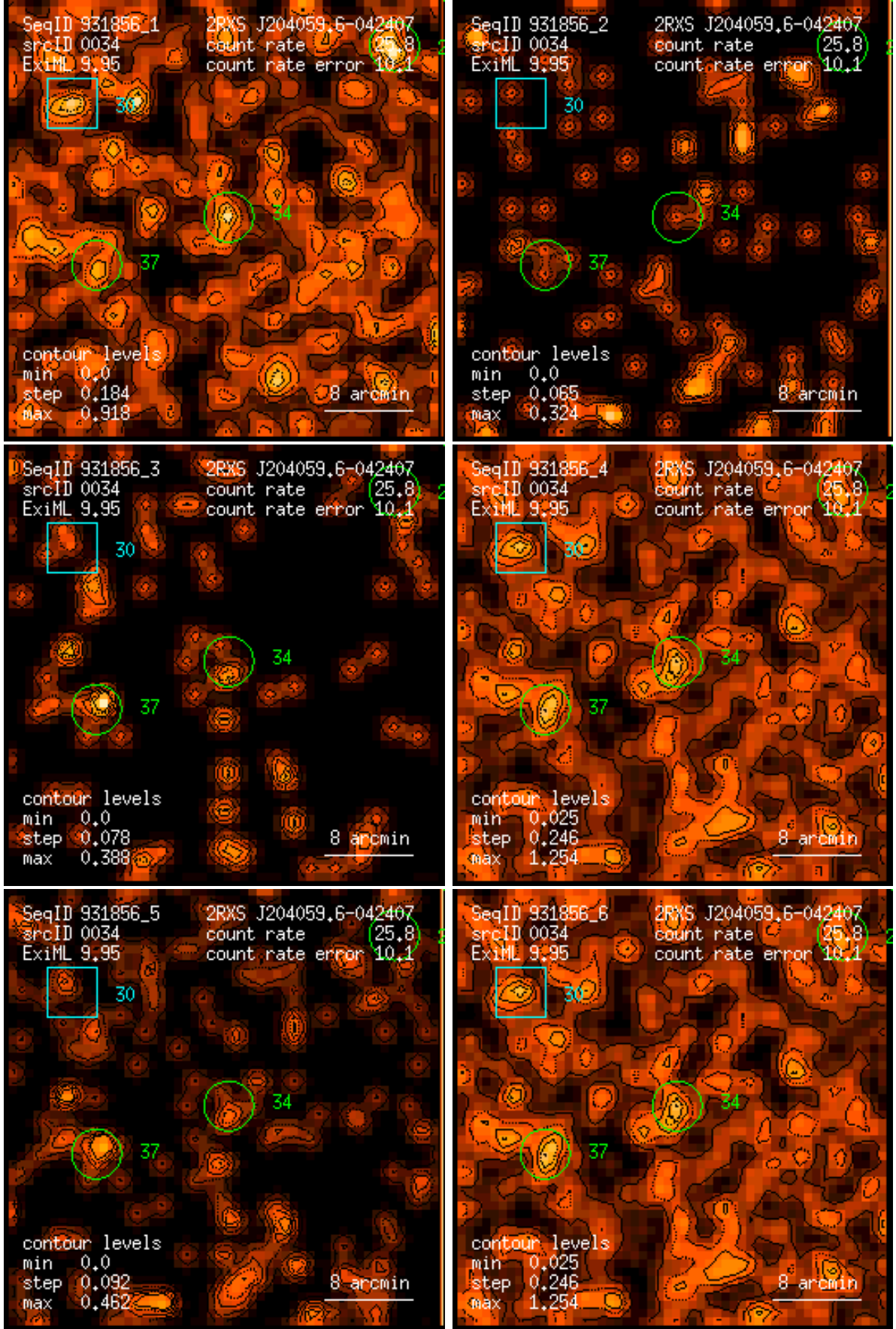
Figure 34: RASS 931856: detection 0034: band rate images, Gaussian filter: (1) PSPC channels 11 – 41, (2) 52 – 90, (3) 91 – 201, (4) 11 – 235, (5) 52 – 201, (6) 11 – 201. Broad band rates in counts/ks. Band rate contour levels in counts/ks/arcmin 2 .
