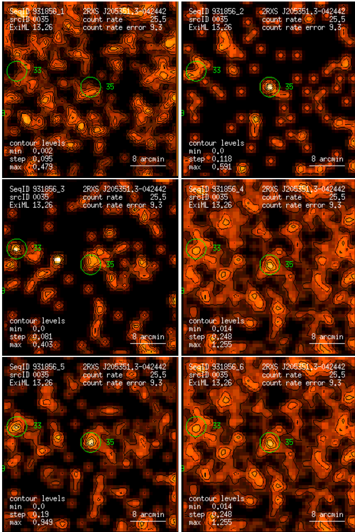
Figure 35: RASS 931856: detection 0035: band rate images, Gaussian filter: (1) PSPC channels 11 – 41, (2) 52 – 90, (3) 91 – 201, (4) 11 – 235, (5) 52 – 201, (6) 11 – 201. Broad band rates in counts/ks. Band rate contour levels in counts/ks/arcmin 2 .
