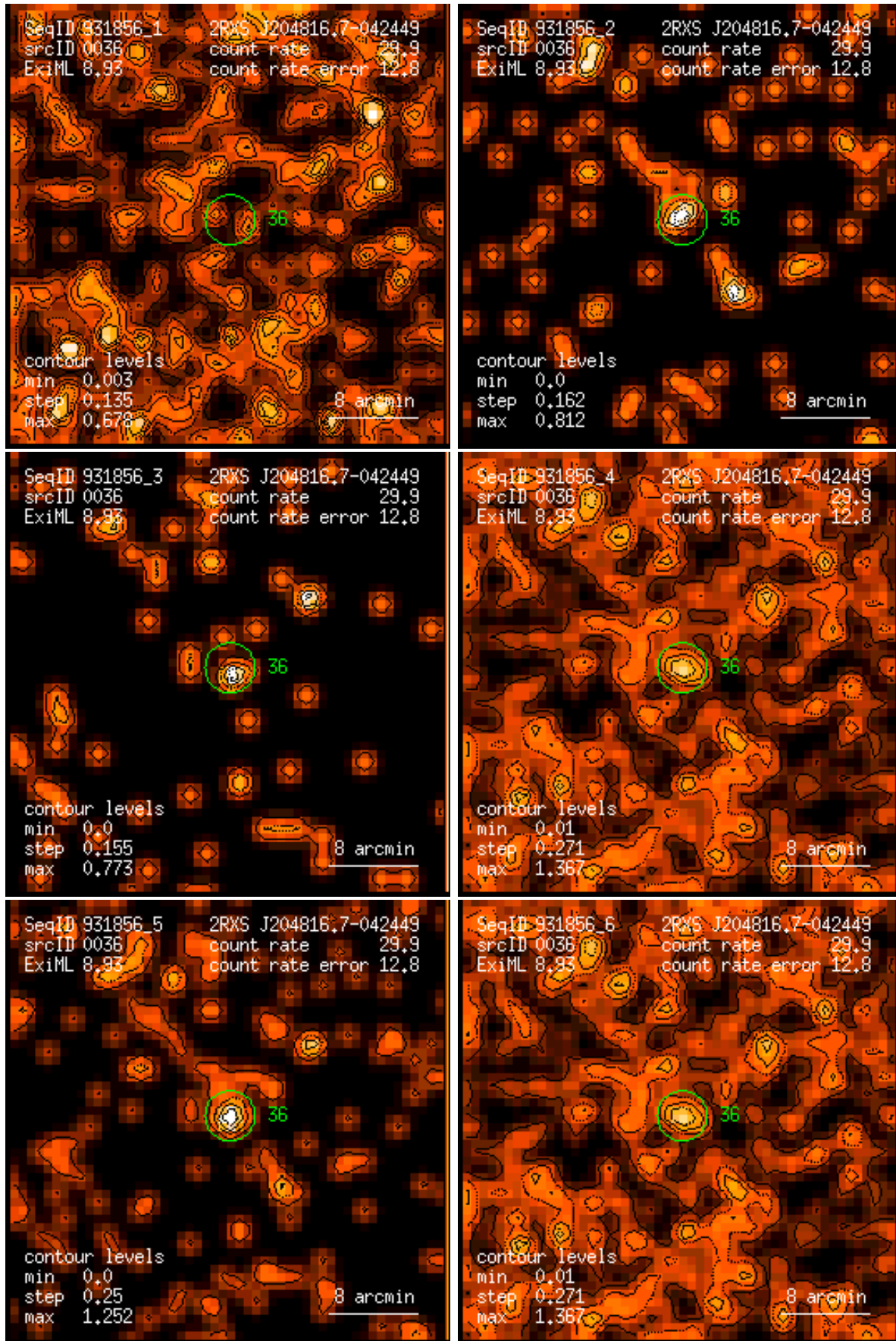
Figure 36: RASS 931856: detection 0036: band rate images, Gaussian filter: (1) PSPC channels 11 – 41, (2) 52 – 90, (3) 91 – 201, (4) 11 – 235, (5) 52 – 201, (6) 11 – 201. Broad band rates in counts/ks. Band rate contour levels in counts/ks/arcmin 2 .
