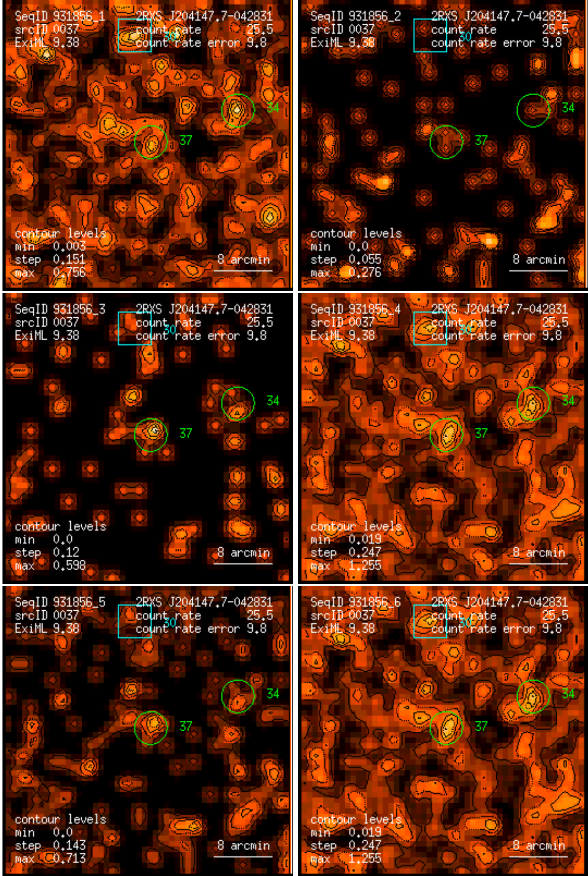
Figure 37: RASS 931856: detection 0037: band rate images, Gaussian filter: (1) PSPC channels 11 – 41, (2) 52 – 90, (3) 91 – 201, (4) 11 – 235, (5) 52 – 201, (6) 11 – 201. Broad band rates in counts/ks. Band rate contour levels in counts/ks/arcmin 2 .
