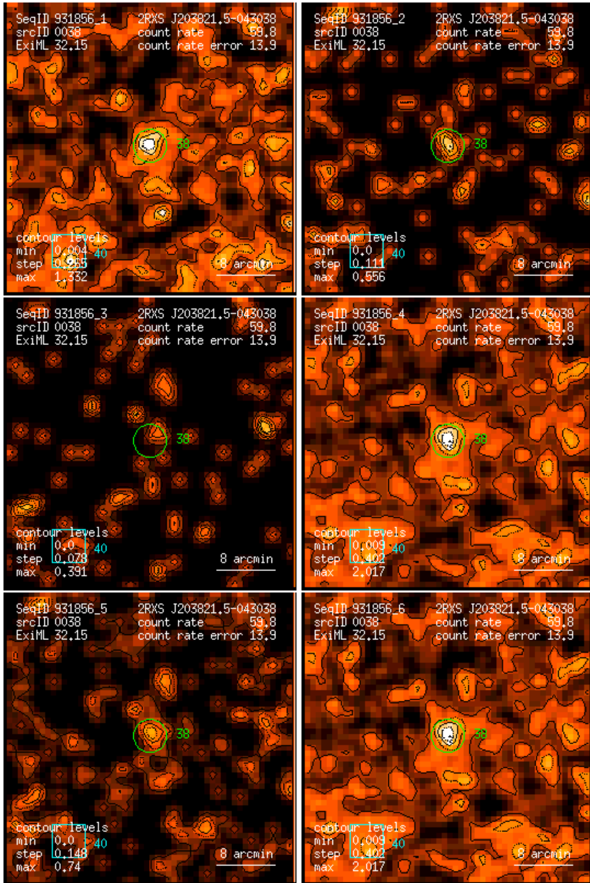
Figure 38: RASS 931856: detection 0038: band rate images, Gaussian filter: (1) PSPC channels 11 – 41, (2) 52 – 90, (3) 91 – 201, (4) 11 – 235, (5) 52 – 201, (6) 11 – 201. Broad band rates in counts/ks. Band rate contour levels in counts/ks/arcmin 2 .
