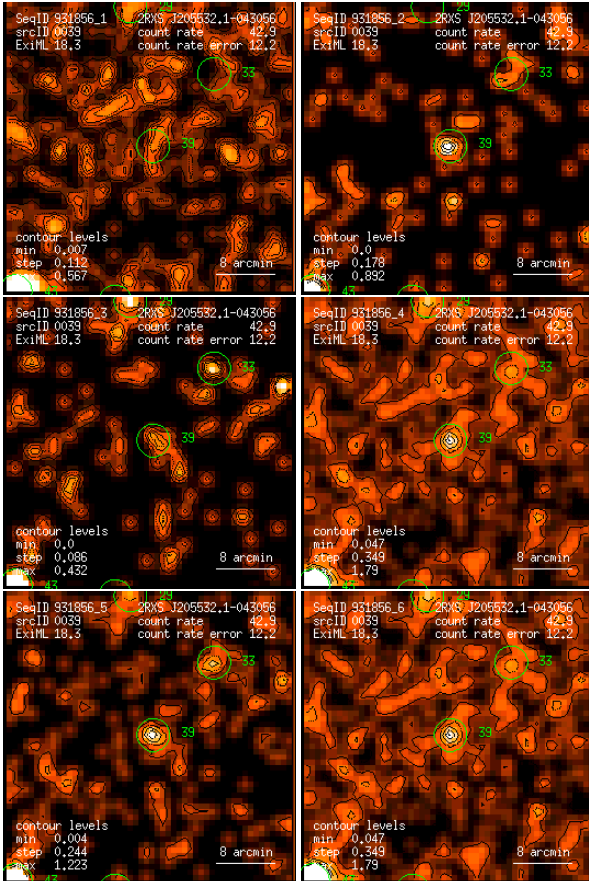
Figure 39: RASS 931856: detection 0039: band rate images, Gaussian filter: (1) PSPC channels 11 – 41, (2) 52 – 90, (3) 91 – 201, (4) 11 – 235, (5) 52 – 201, (6) 11 – 201. Broad band rates in counts/ks. Band rate contour levels in counts/ks/arcmin 2 .
