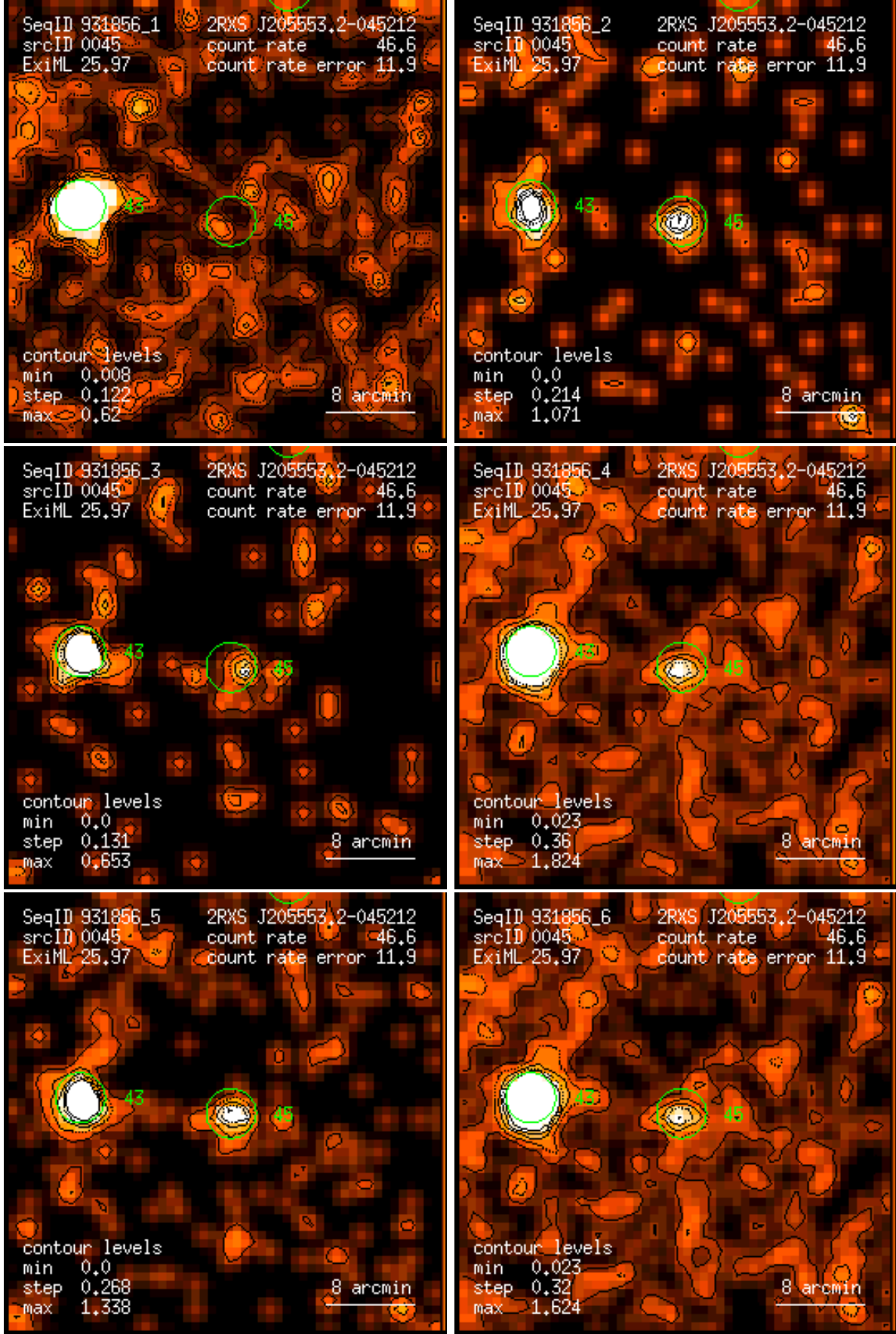
Figure 45: RASS 931856: detection 0045: band rate images, Gaussian filter: (1) PSPC channels 11 – 41, (2) 52 – 90, (3) 91 – 201, (4) 11 – 235, (5) 52 – 201, (6) 11 – 201. Broad band rates in counts/ks. Band rate contour levels in counts/ks/arcmin 2 .
