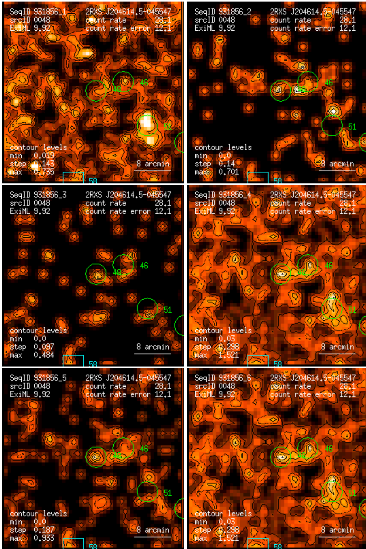
Figure 48: RASS 931856: detection 0048: band rate images, Gaussian filter: (1) PSPC channels 11 – 41, (2) 52 – 90, (3) 91 – 201, (4) 11 – 235, (5) 52 – 201, (6) 11 – 201. Broad band rates in counts/ks. Band rate contour levels in counts/ks/arcmin 2 .
