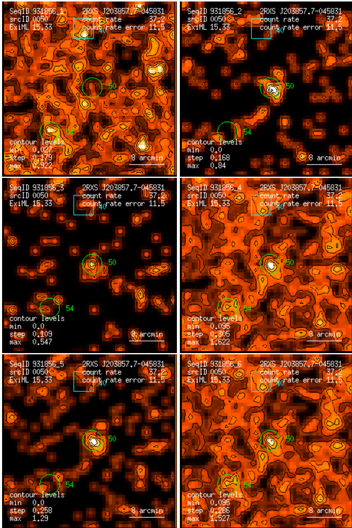
Figure 50: RASS 931856: detection 0050: band rate images, Gaussian filter: (1) PSPC channels 11 – 41, (2) 52 – 90, (3) 91 – 201, (4) 11 – 235, (5) 52 – 201, (6) 11 – 201. Broad band rates in counts/ks. Band rate contour levels in counts/ks/arcmin 2 .
