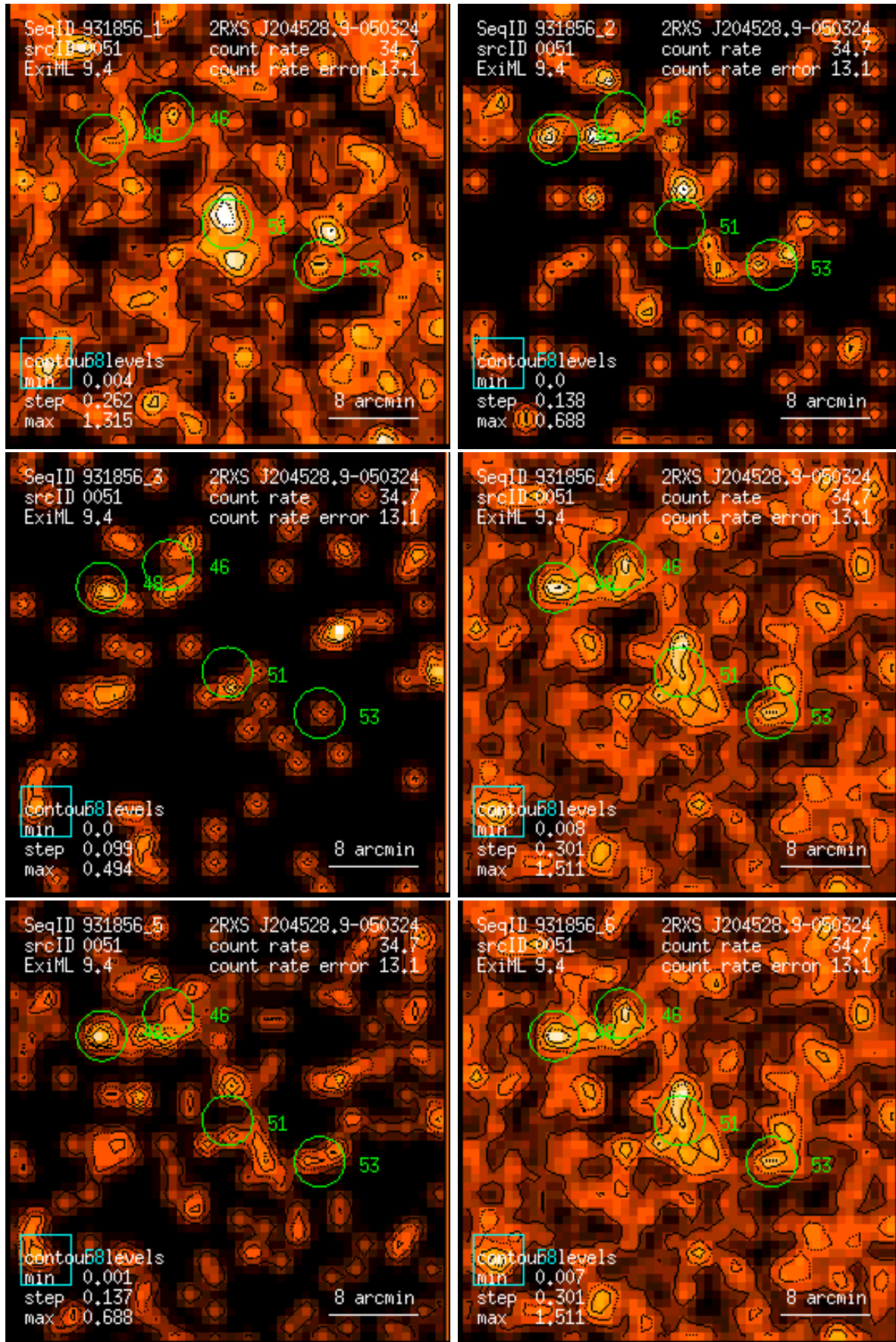
Figure 51: RASS 931856: detection 0051: band rate images, Gaussian filter: (1) PSPC channels 11 – 41, (2) 52 – 90, (3) 91 – 201, (4) 11 – 235, (5) 52 – 201, (6) 11 – 201. Broad band rates in counts/ks. Band rate contour levels in counts/ks/arcmin 2 .
