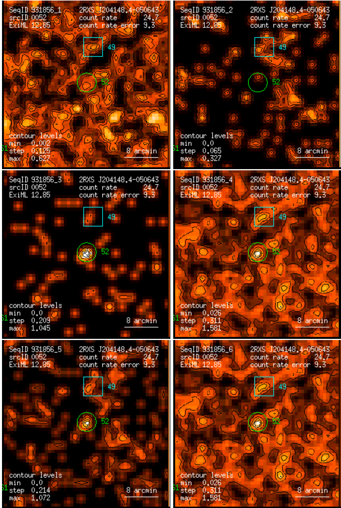
Figure 52: RASS 931856: detection 0052: band rate images, Gaussian filter: (1) PSPC channels 11 – 41, (2) 52 – 90, (3) 91 – 201, (4) 11 – 235, (5) 52 – 201, (6) 11 – 201. Broad band rates in counts/ks. Band rate contour levels in counts/ks/arcmin 2 .
